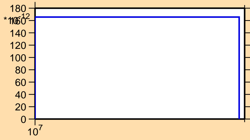
\sigma vs. E for ^{76}\text{Br}(n,\text{pt})
