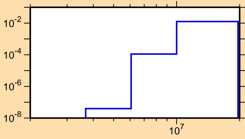
\sigma vs. E for ^{76}\text{Br}(n,d)
