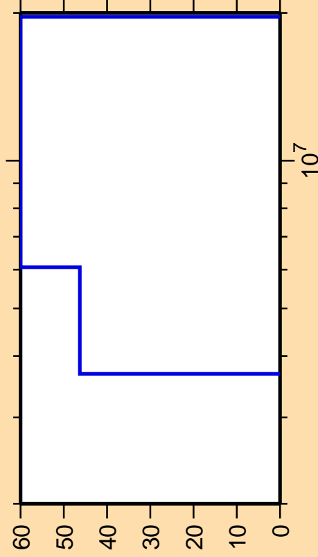
\Delta\sigma/\sigma vs. E for ^{76}\text{Br}(n,d)
