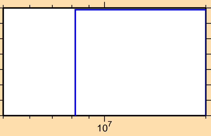
\sigma vs. E for ^{76}\text{Br}(n,\text{He}3)
