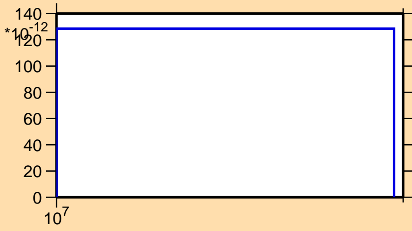
\sigma vs. E for ^{77}\text{Br}(n,pd)
