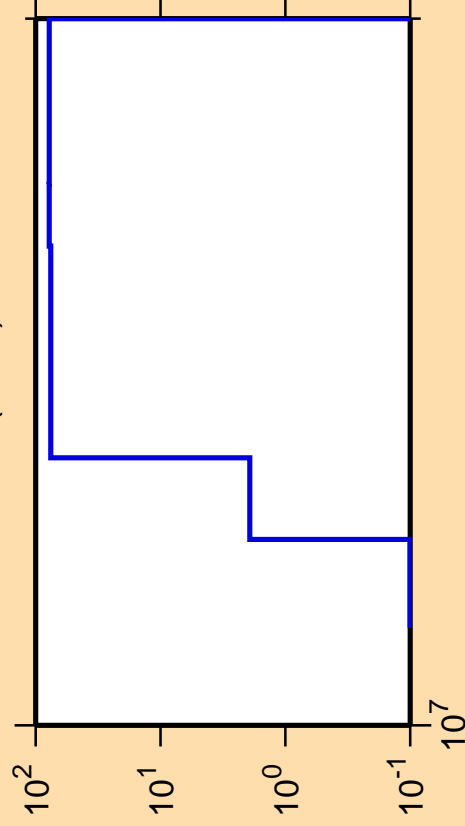
\Delta\sigma/\sigma vs. E for ^{78}\text{Br}(n,nd)
