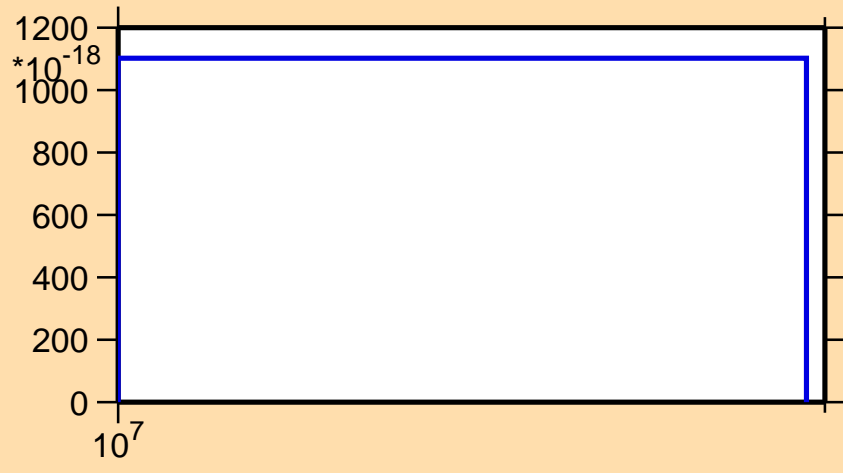
\sigma vs. E for ^{78}\text{Br} (mt 34)
