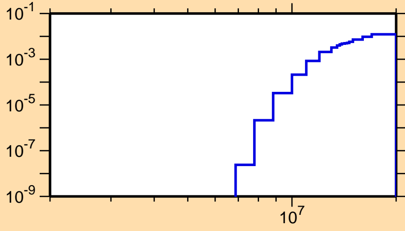
\sigma vs. E for ^{80}\text{Br}(n,d)
