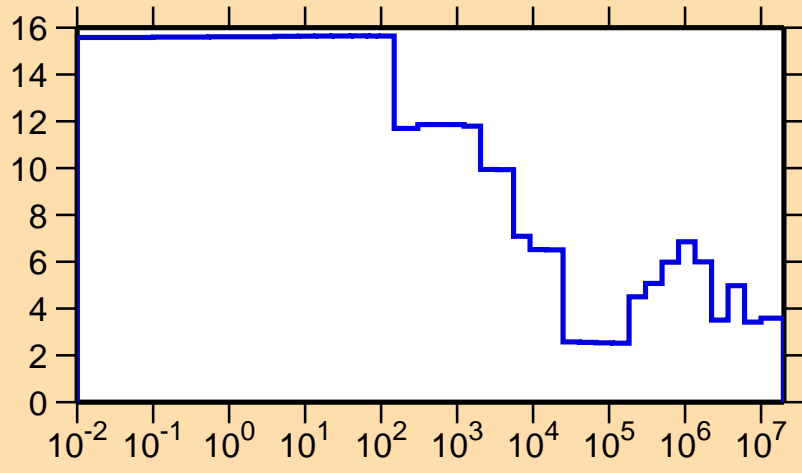
\Delta\sigma/\sigma vs. E for ^{80}\text{Br}(n,\text{el.})
