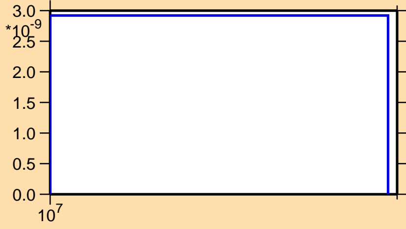
\sigma vs. E for ^{80}\text{Br}(n,\text{He}3)
