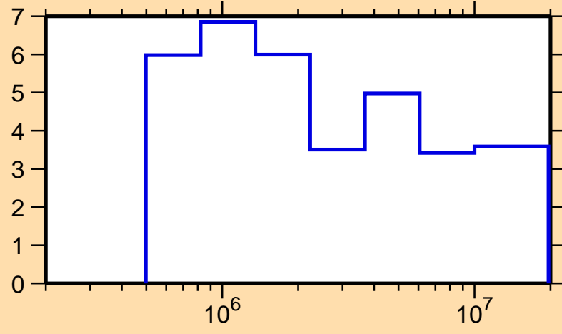
\Delta\sigma/\sigma vs. E for ^{80}\text{Br}(n,\text{el.})
