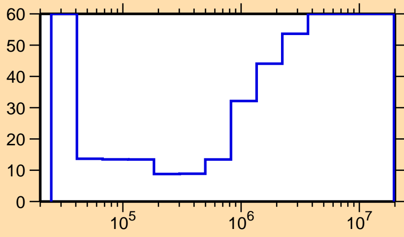
\Delta\sigma/\sigma vs. E for ^{80}\text{Br}(n,n_1)
