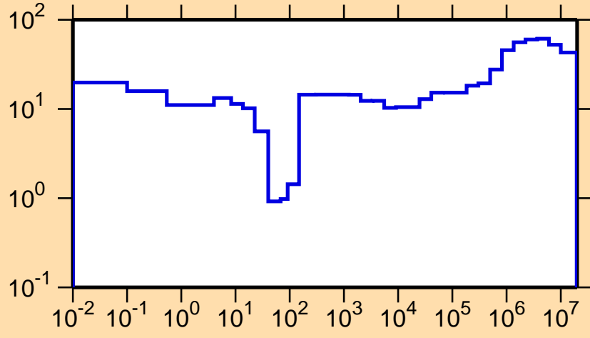
\Delta\sigma/\sigma vs. E for ^{80}\text{Br}(n,\gamma)
