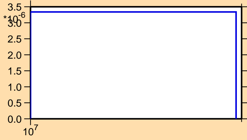
\sigma vs. E for ^{80}\text{Br}(n,\text{nd})
