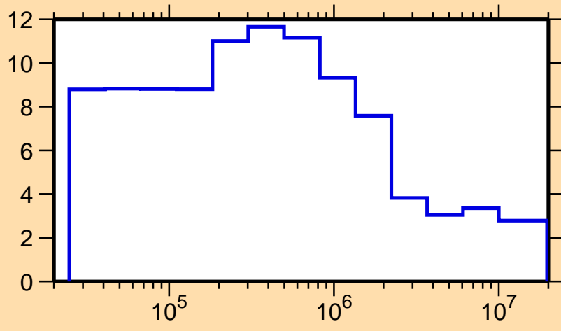
\Delta\sigma/\sigma vs. E for ^{80}\text{Br}(n,\text{nonel.})
