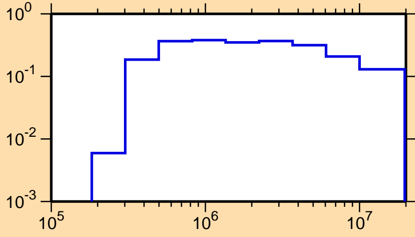
\sigma vs. E for ^{80}\text{Br}(n,n_4)
