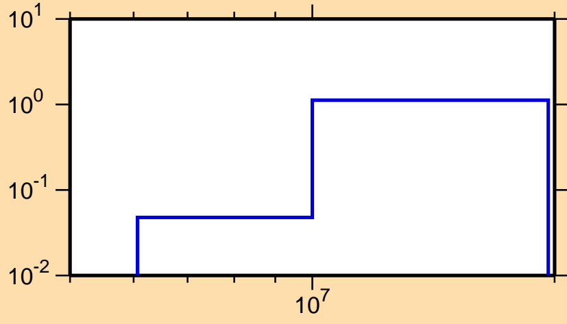
\sigma vs. E for ^{80}\text{Br}(n,2n)
