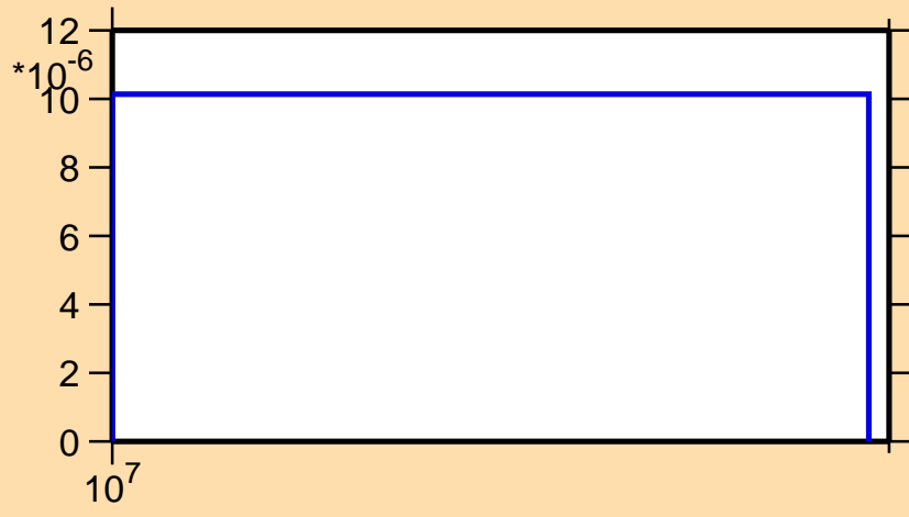
\sigma vs. E for ^{80}\text{Br}(n,2np)
