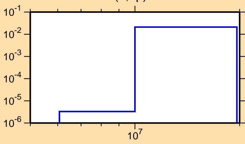
\sigma vs. E for ^{80}\text{Br}(n,np)
