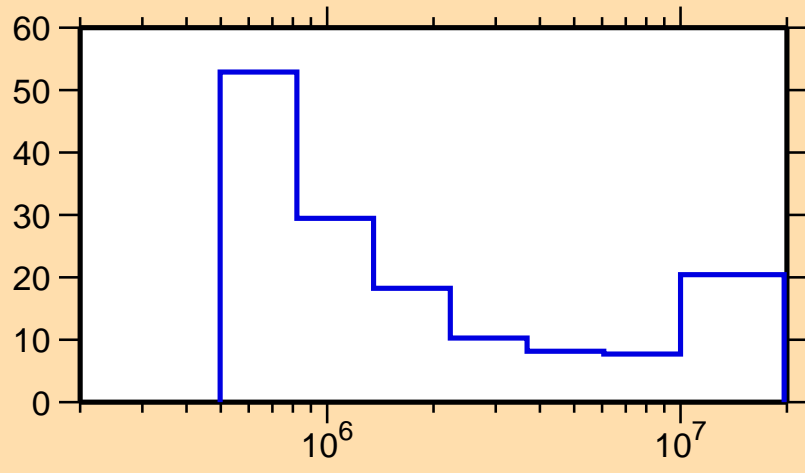
\Delta\sigma/\sigma vs. E for ^{80}\text{Br}(n,n\text{cont.})
