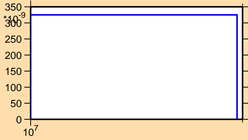
\sigma vs. E for ^{80}\text{Br}(n,3n)
