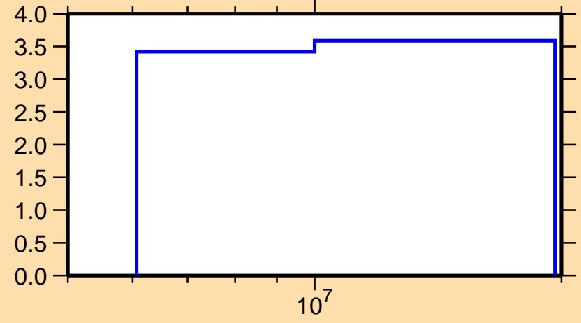
\Delta\sigma/\sigma vs. E for ^{80}\text{Br}(n,\text{el.})
