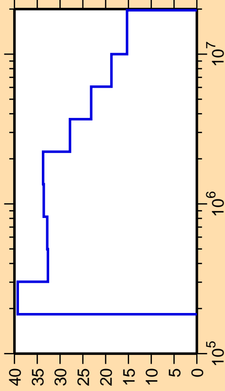
\Delta\sigma/\sigma vs. E for ^{80}\text{Br}(n,n_4)
