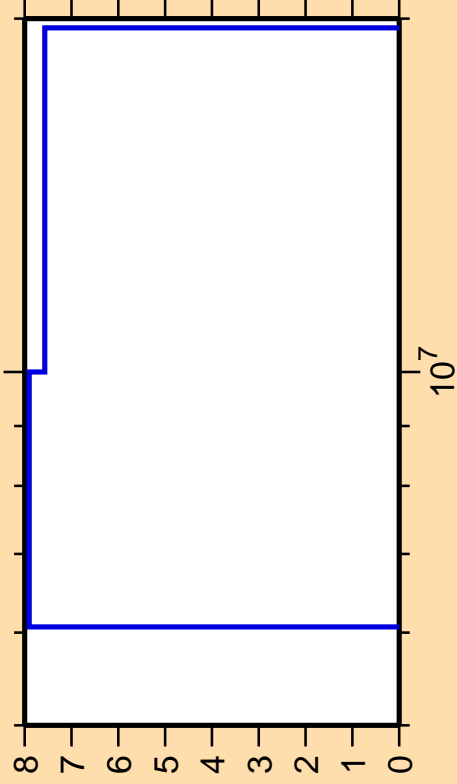
\Delta\sigma/\sigma vs. E for ^{80}\text{Br}(n,2n)
