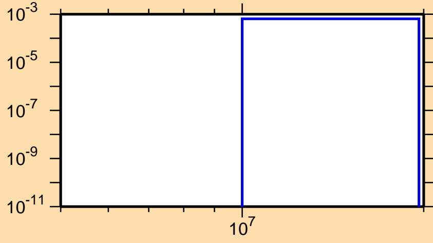
\sigma vs. E for ^{80}\text{Br}(n,n\alpha)
