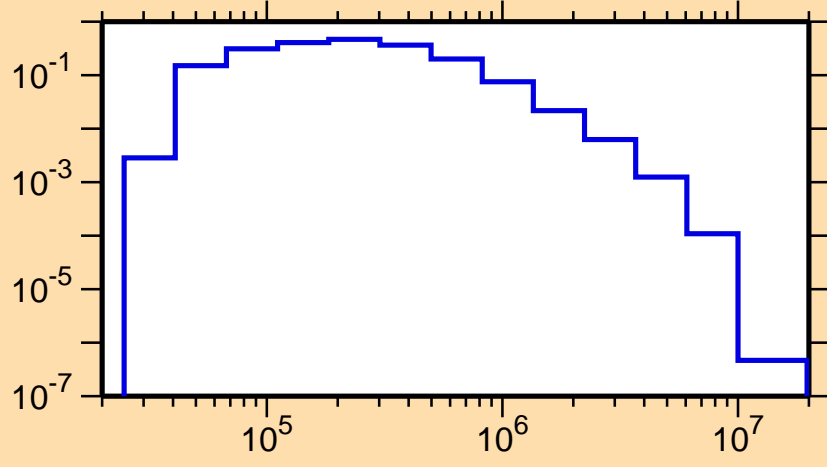
\sigma vs. E for ^{80}\text{Br}(n,n_1)
