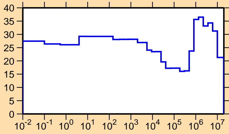
\Delta\sigma/\sigma vs. E for ^{80}\text{Br}(n,p)
