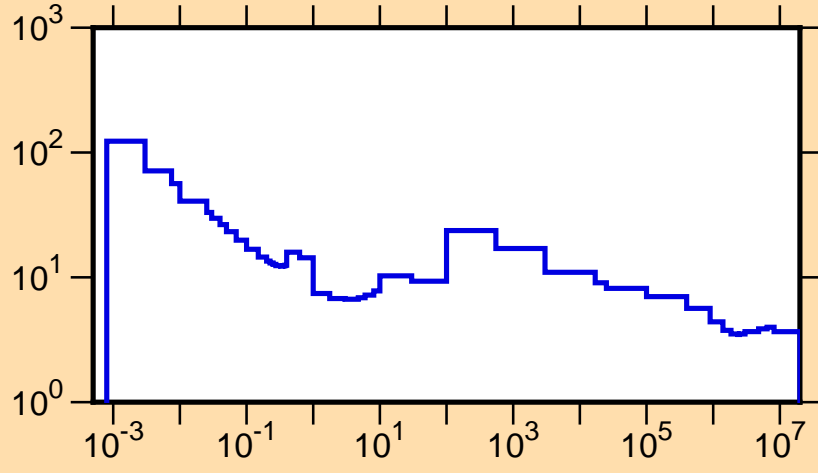
\sigma vs. E for ^{80}\text{Br}(n,\text{tot.})
