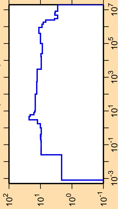
\Delta\sigma/\sigma vs. E for ^{80}\text{Br}(n,\text{nonel.})
