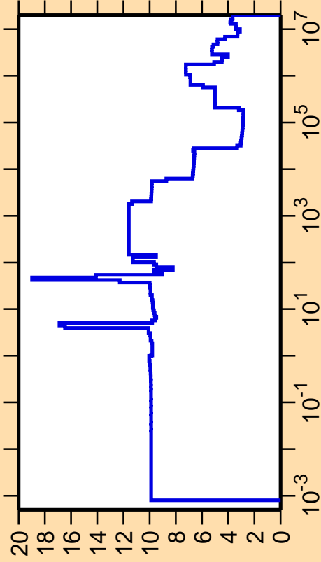
\Delta\sigma/\sigma vs. E for ^{80}\text{Br}(n,\text{el.})
