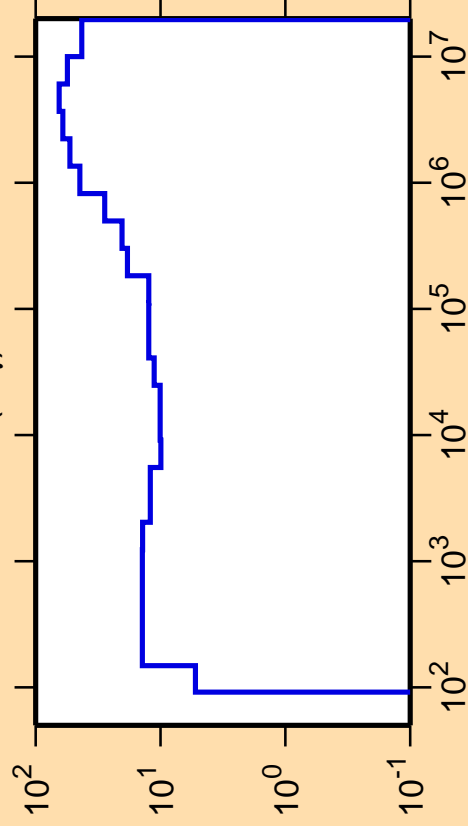
\Delta\sigma/\sigma vs. E for ^{80}\text{Br}(n,\gamma)
