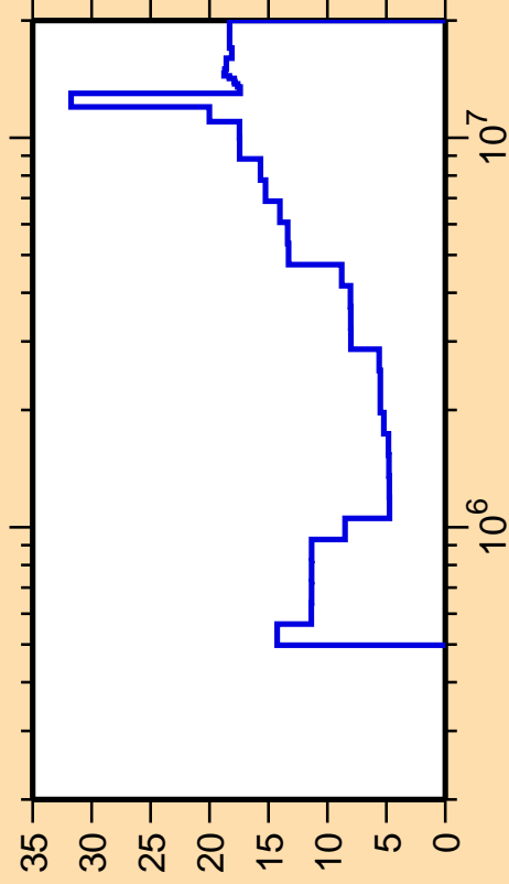
\Delta\sigma/\sigma vs. E for ^{81}\text{Br}(n,n_3)
