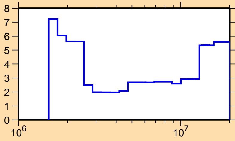
\Delta\sigma/\sigma vs. E for ^{81}\text{Br}(n,\text{inel.})
