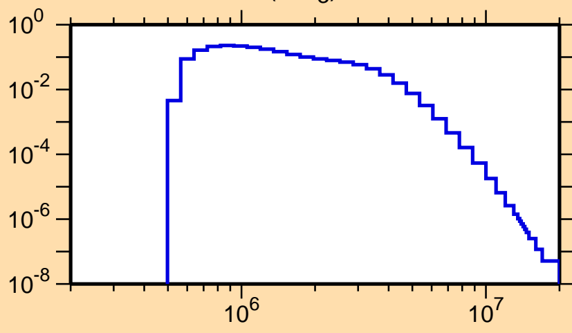
\sigma vs. E for ^{81}\text{Br}(n,n_3)
