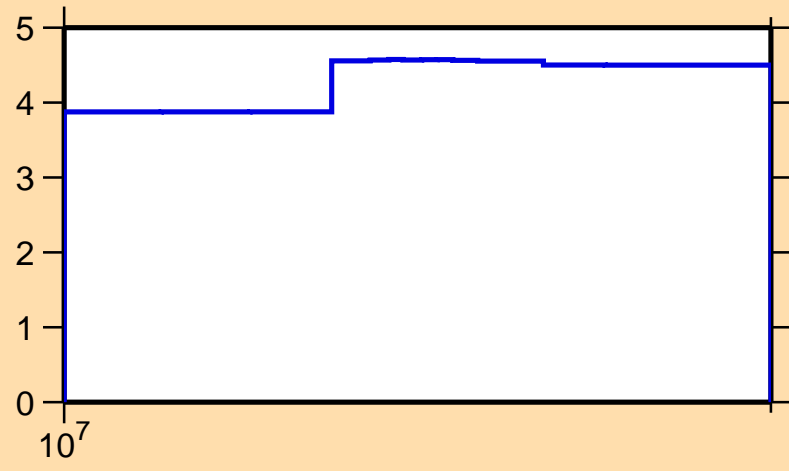
\Delta\sigma/\sigma vs. E for ^{81}\text{Br}(n,\text{el.})
