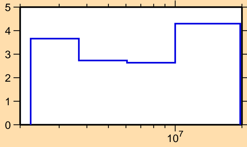
\Delta\sigma/\sigma vs. E for ^{81}\text{Br}(n,n\text{cont.})
