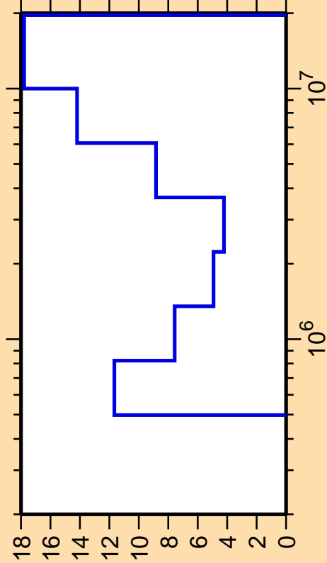
\Delta\sigma/\sigma vs. E for ^{81}\text{Br}(n,n_4)
