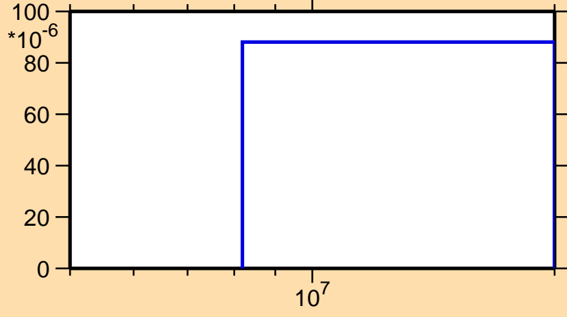
\sigma vs. E for ^{81}\text{Br}(n,t)
