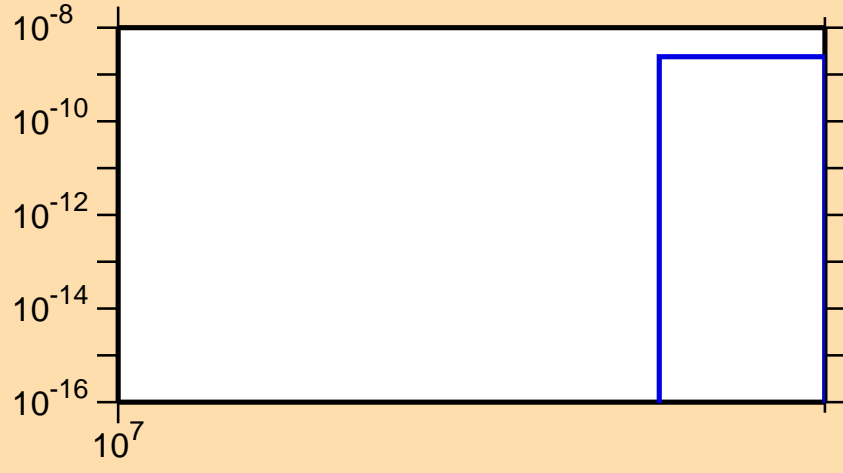
\sigma vs. E for ^{82}\text{Br}(n,nt)
