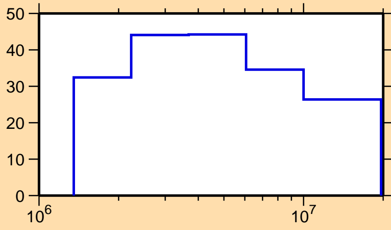
\Delta\sigma/\sigma vs. E for ^{82}\text{Br}(n,p)
