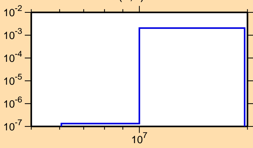
\sigma vs. E for ^{82}\text{Br}(n,d)
