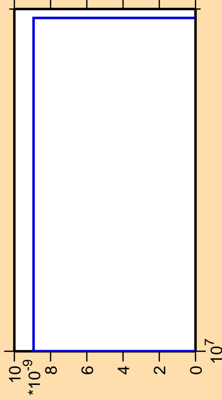
\Delta\sigma/\sigma vs. E for ^{82}\text{Br} (mt 34)
