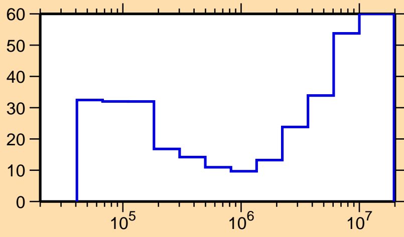
\Delta\sigma/\sigma vs. E for ^{82}\text{Br}(n,n_1)
