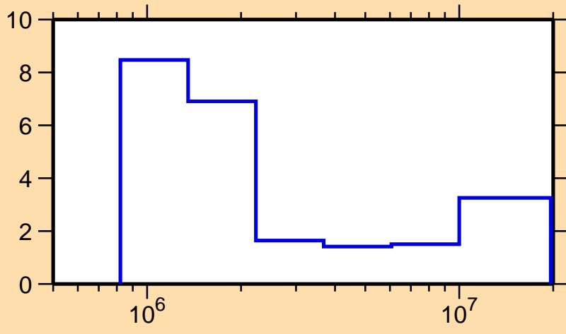
\Delta\sigma/\sigma vs. E for ^{82}\text{Br}(n,\text{tot.})
