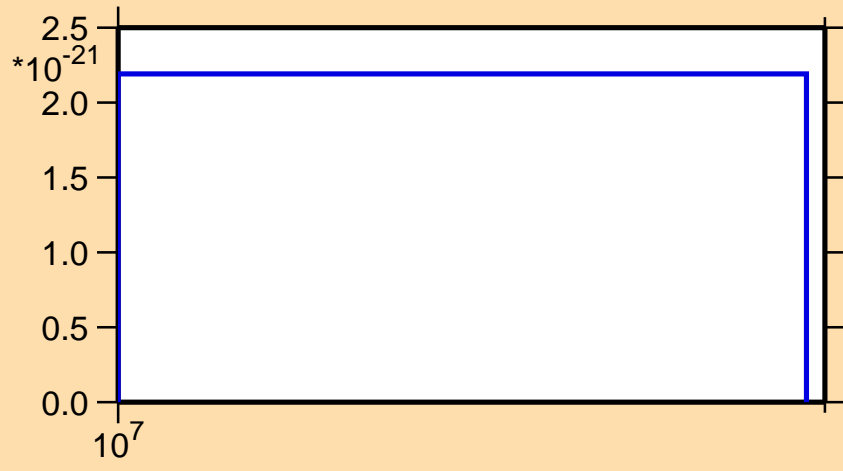
\sigma vs. E for ^{82}\text{Br} (mt 34)
