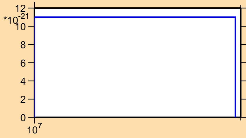
\sigma vs. E for ^{82}\text{Br}(n,\text{pt})
