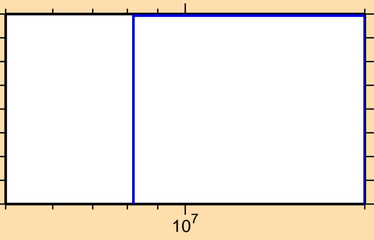
\sigma vs. E for ^{82}\text{Br}(n,2np)
