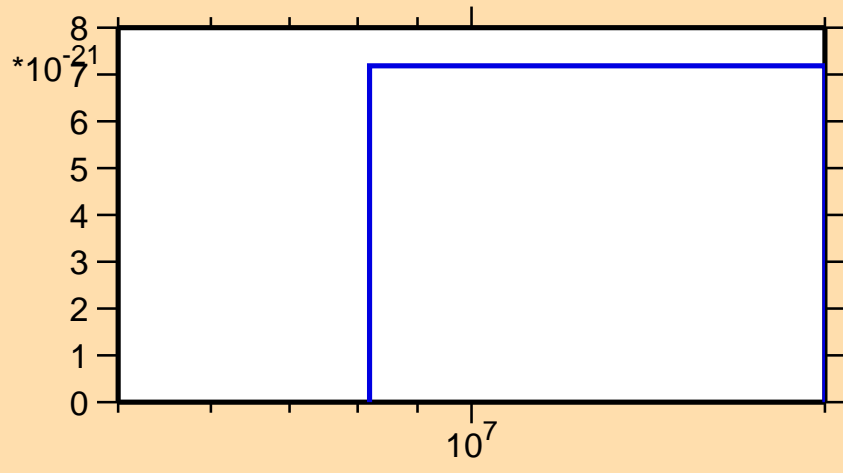
\sigma vs. E for ^{82}\text{Br} (mt 34)
