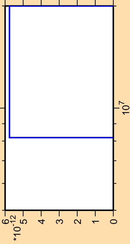
\Delta\sigma/\sigma vs. E for ^{82}\text{Br}(n,\text{pt})
