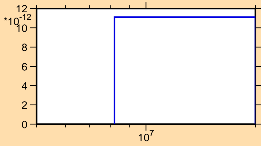
\sigma vs. E for ^{82}\text{Br}(n,\text{He}3)
