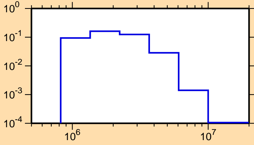
\sigma vs. E for ^{83}\text{Br}(n,n_3)
