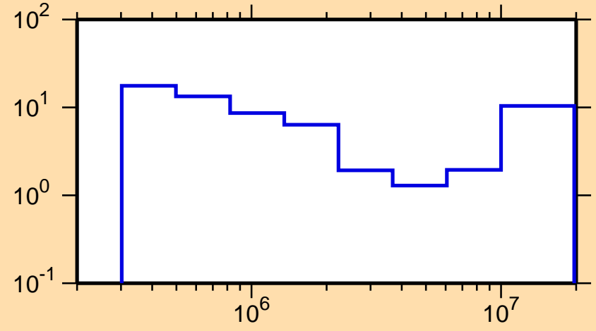
\Delta\sigma/\sigma vs. E for ^{83}\text{Br}(n,\text{inel.})
