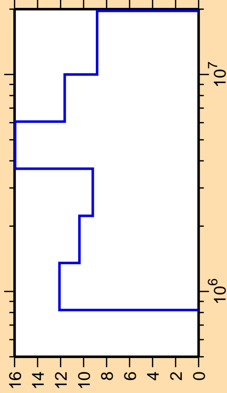
\Delta\sigma/\sigma vs. E for ^{83}\text{Br}(n,n_3)
