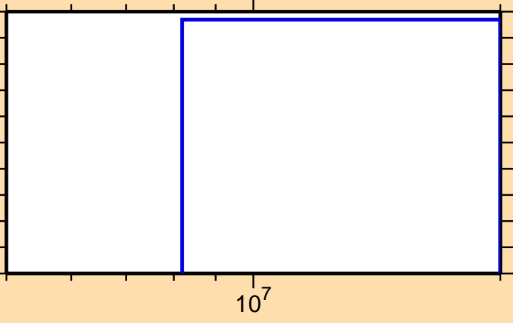
\sigma vs. E for ^{83}\text{Br}(n,nt)
