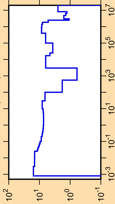
\Delta\sigma/\sigma vs. E for ^{83}\text{Br}(n,\text{tot.})
