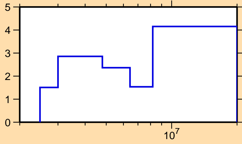
\Delta\sigma/\sigma vs. E for ^{83}\text{Br}(n,\text{el.})
