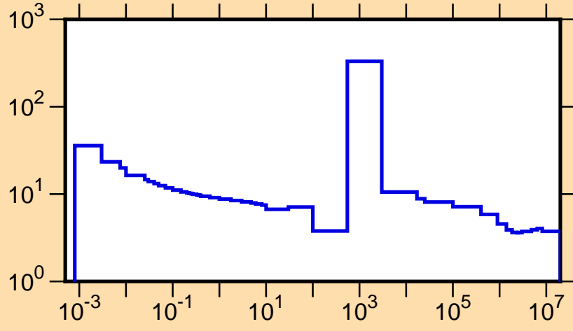
\sigma vs. E for ^{83}\text{Br}(n,\text{tot.})
