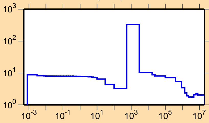
\sigma vs. E for ^{83}\text{Br}(n,\text{el.})
