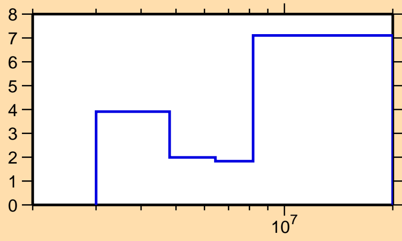
\Delta\sigma/\sigma vs. E for ^{83}\text{Br}(n,n\text{cont.})
