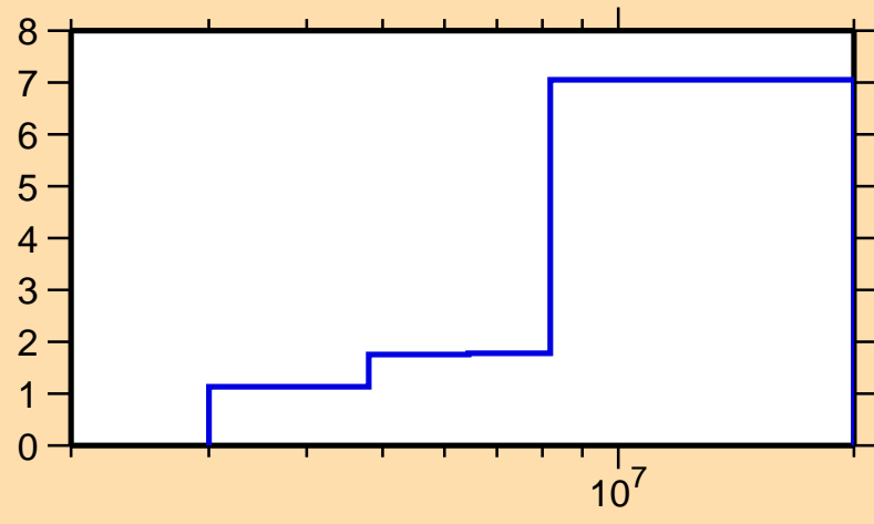
\Delta\sigma/\sigma vs. E for ^{83}\text{Br}(n,\text{inel.})
