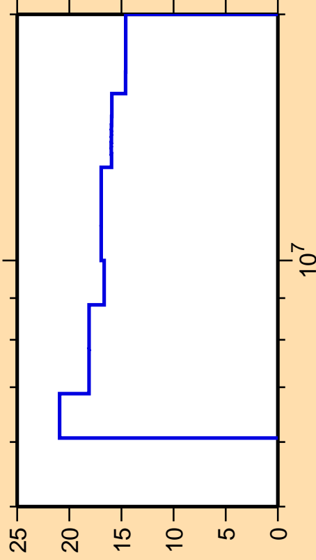
\Delta\sigma/\sigma vs. E for ^{84}\text{Br}(n,p)
