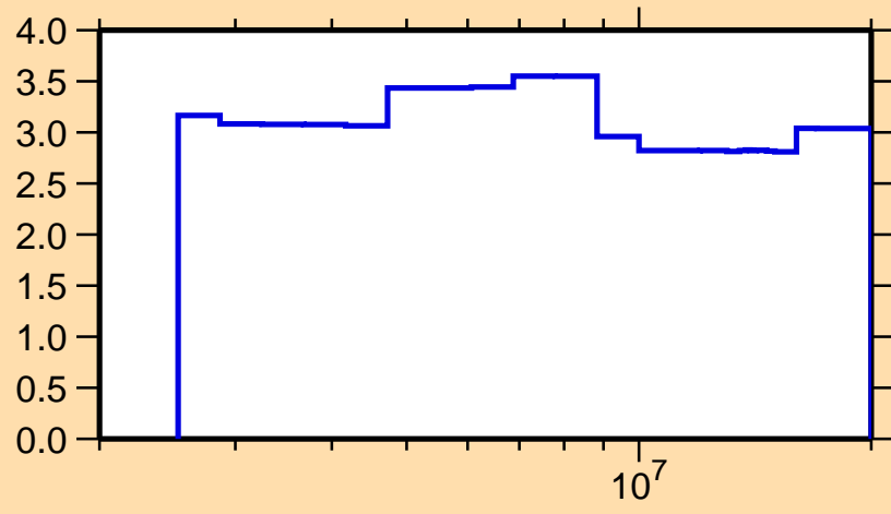
\Delta\sigma/\sigma vs. E for ^{84}\text{Br}(n,n\text{onel.})
