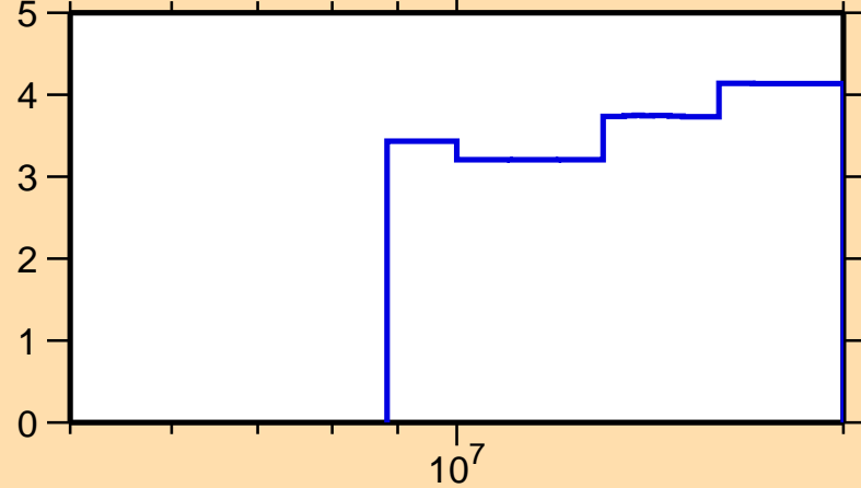
\Delta\sigma/\sigma vs. E for ^{85}\text{Br}(n,\text{nonel.})
