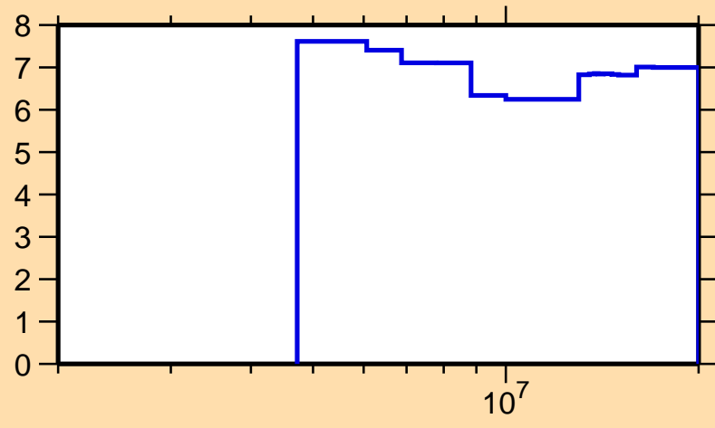
\Delta\sigma/\sigma vs. E for ^{86}\text{Br}(n,\text{nonel.})
