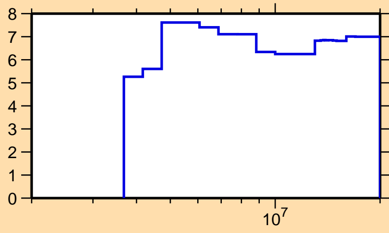
\Delta\sigma/\sigma vs. E for ^{86}\text{Br}(n,n\text{onel.})
