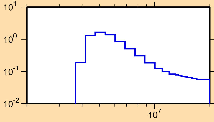
\sigma vs. E for ^{86}\text{Br}(n,n\text{cont.})
