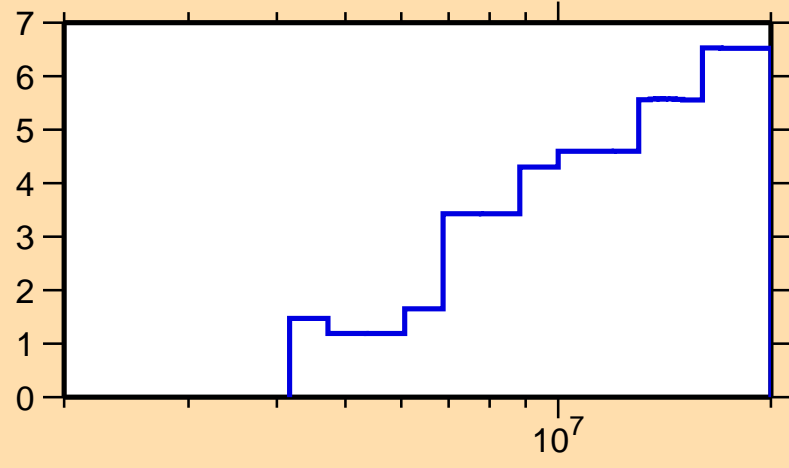
\Delta\sigma/\sigma vs. E for ^{86}\text{Br}(n,\text{tot.})
