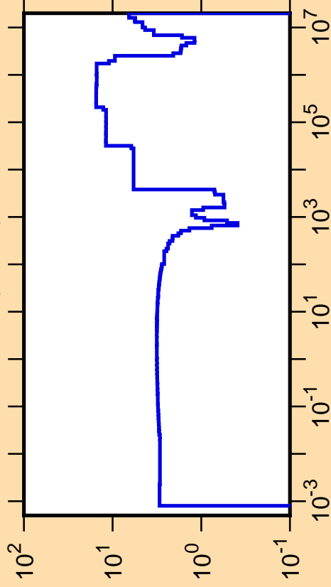
\Delta\sigma/\sigma vs. E for ^{86}\text{Br}(n,\text{tot.})
