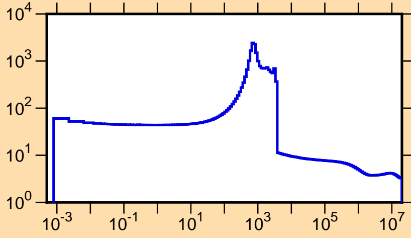
\sigma vs. E for ^{86}\text{Br}(n,\text{tot.})
