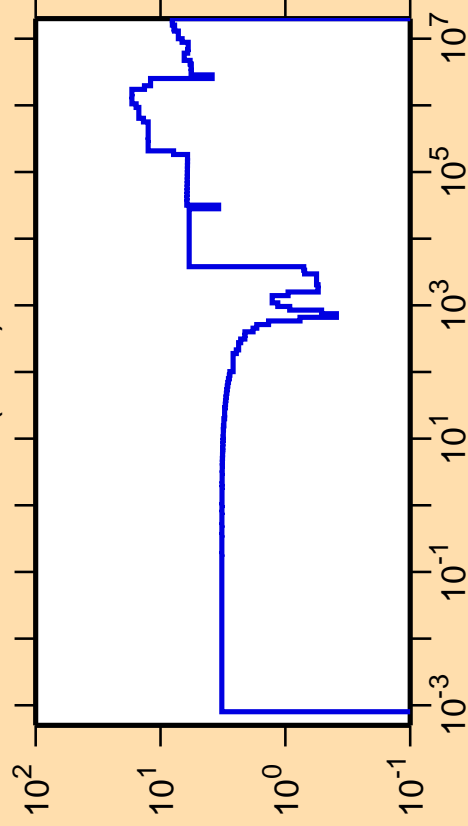
\Delta\sigma/\sigma vs. E for ^{86}\text{Br}(n,\text{el.})
