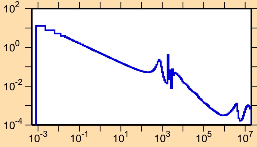
\sigma vs. E for ^{86}\text{Br}(n,\gamma)
