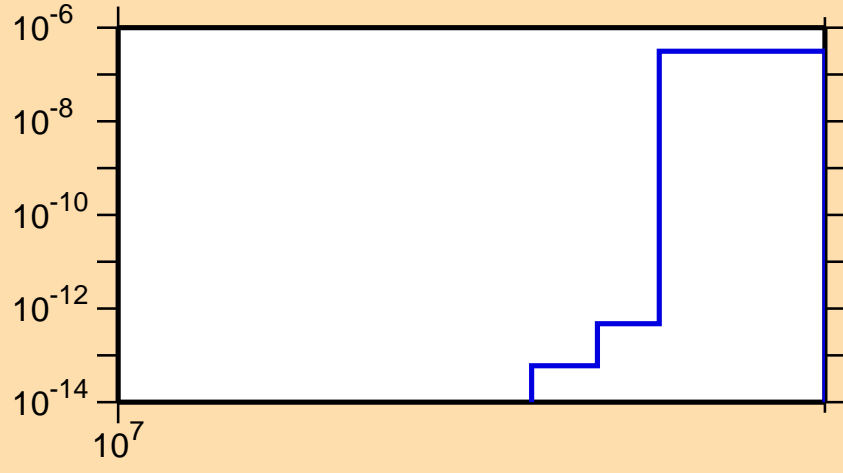
\sigma vs. E for ^{86}\text{Br}(n,nt)
