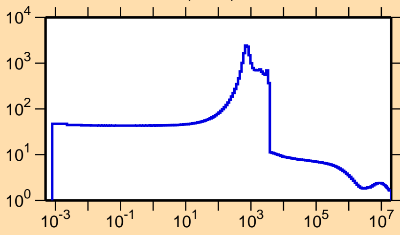
\sigma vs. E for ^{86}\text{Br}(n,\text{el.})
