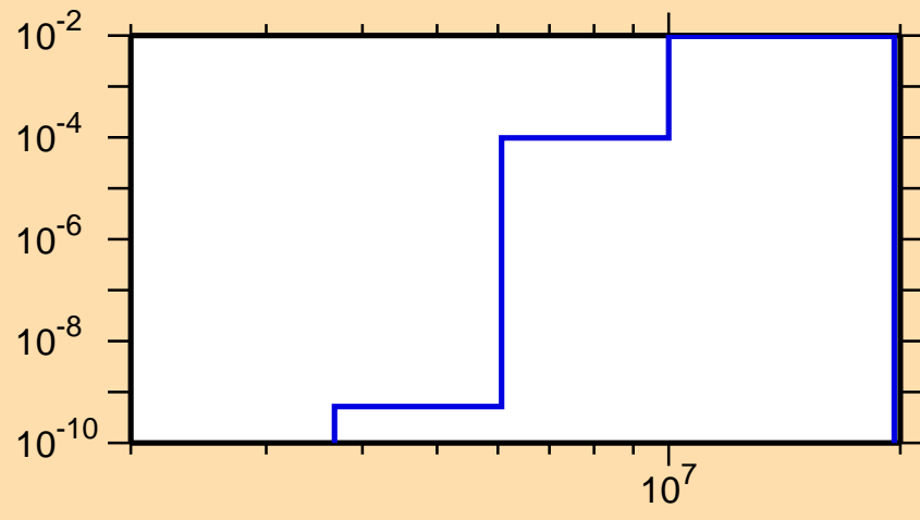
\sigma vs. E for ^{86}\text{Br}(n,p)
