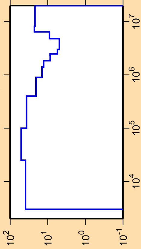
\Delta\sigma/\sigma vs. E for ^{86}\text{Br}(n,\text{inel.})
