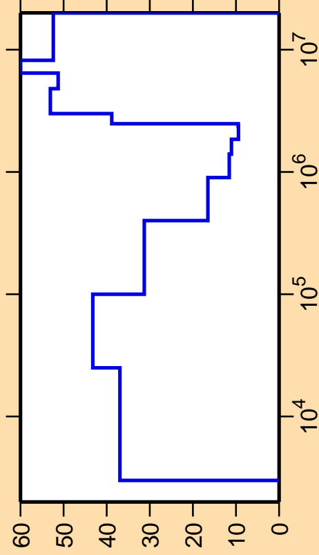
\Delta\sigma/\sigma vs. E for ^{86}\text{Br}(n,n_1)
