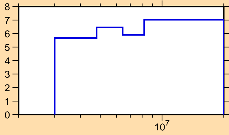
\Delta\sigma/\sigma vs. E for ^{86}\text{Br}(n,\text{el.})
