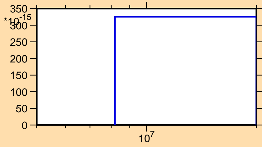
\sigma vs. E for ^{86}\text{Br}(n,2n\alpha)
