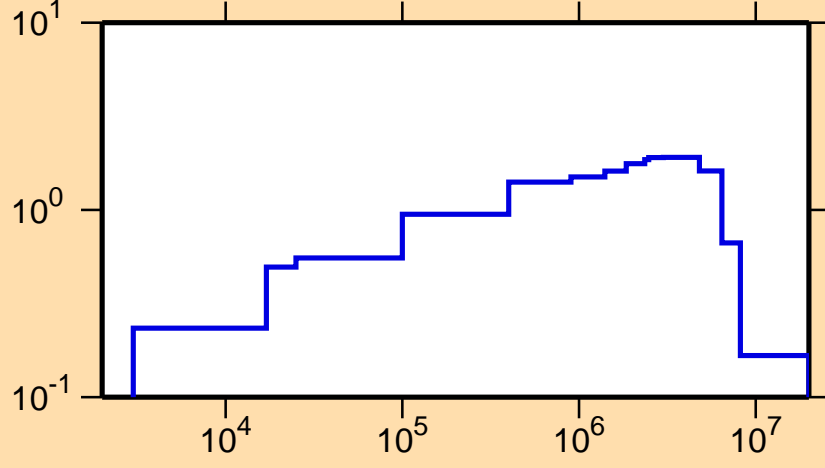
\sigma vs. E for ^{86}\text{Br}(n,\text{inel.})
