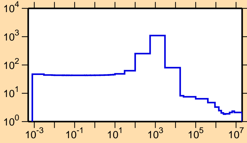
\sigma vs. E for ^{86}\text{Br}(n,\text{el.})
