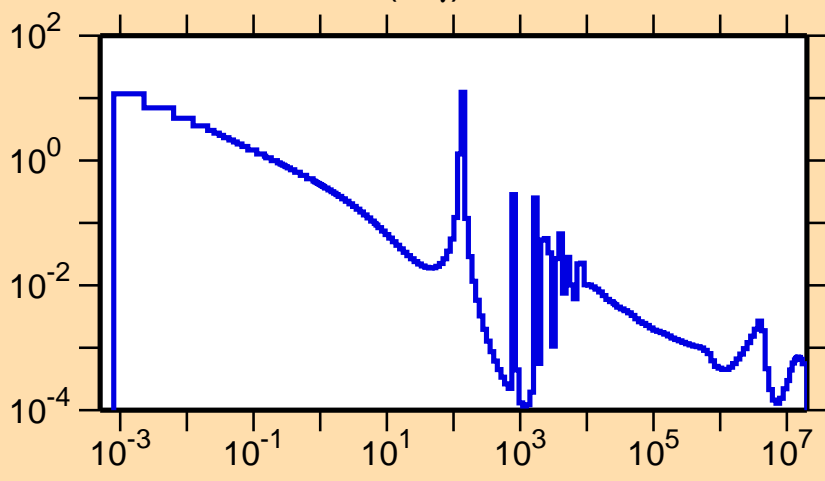
\sigma vs. E for ^{87}\text{Br}(n,\gamma)
