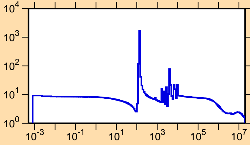
\sigma vs. E for ^{87}\text{Br}(n,\text{el.})
