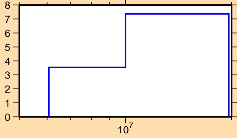
\Delta\sigma/\sigma vs. E for ^{87}\text{Br}(n,tot.)
