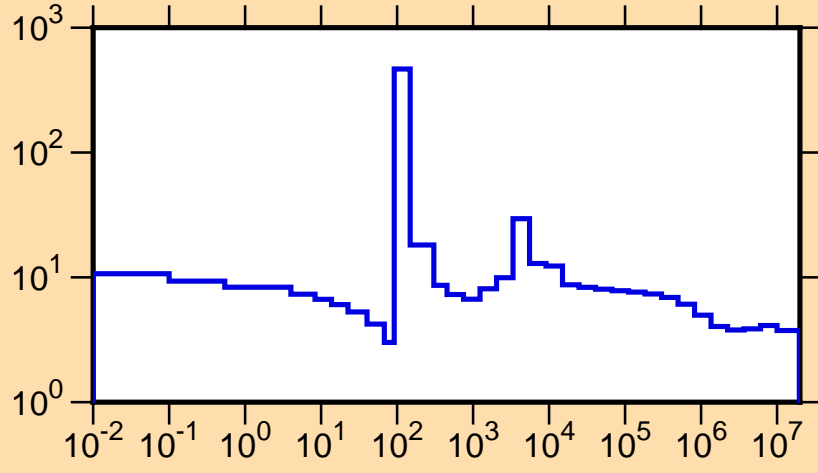
\sigma vs. E for ^{87}\text{Br}(n,\text{tot.})
