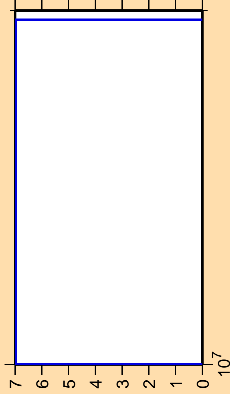
\Delta\sigma/\sigma vs. E for ^{87}\text{Br}(n,2np)
