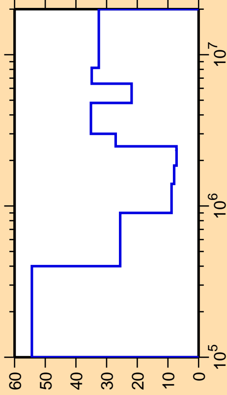
\Delta\sigma/\sigma vs. E for ^{87}\text{Br}(n,n_2)
