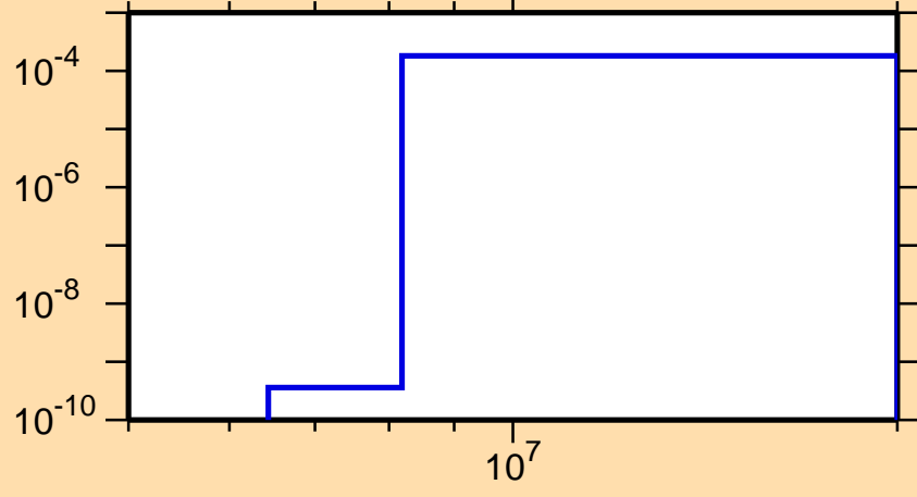
\sigma vs. E for ^{87}\text{Br}(n,\alpha)
