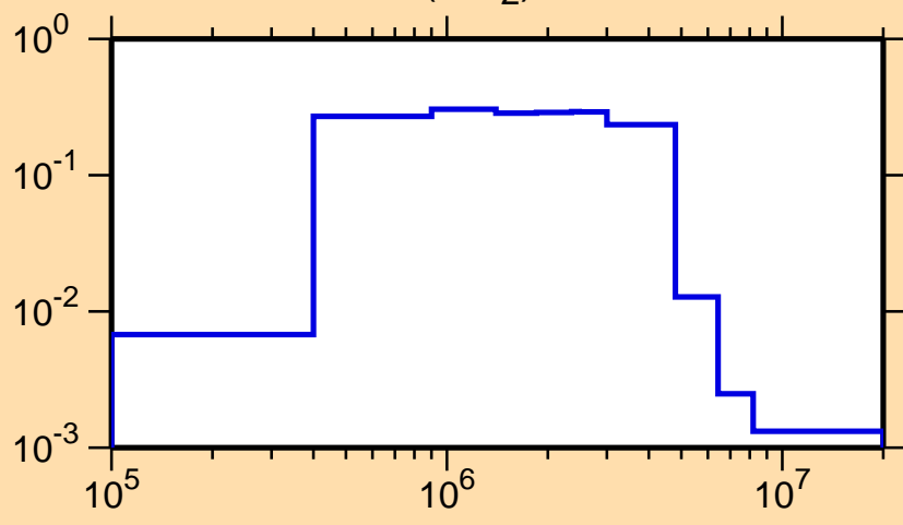
\sigma vs. E for ^{87}\text{Br}(n,n_2)
