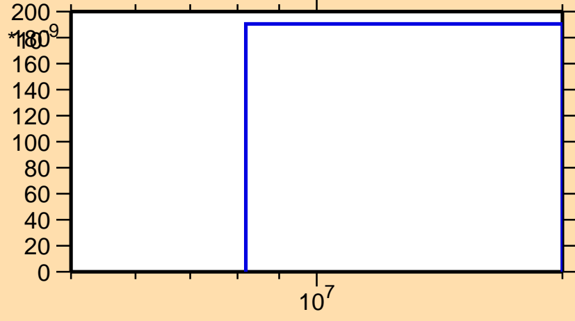
\sigma vs. E for ^{87}\text{Br}(n,nt)
