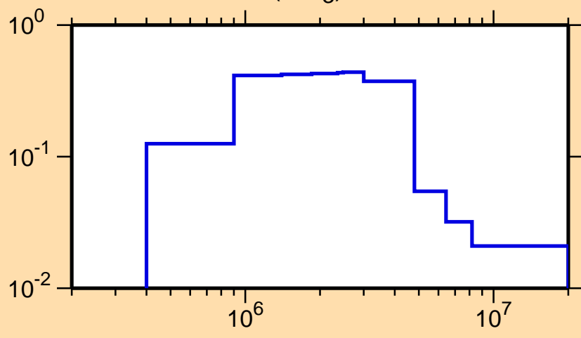
\sigma vs. E for ^{87}\text{Br}(n,n_3)
