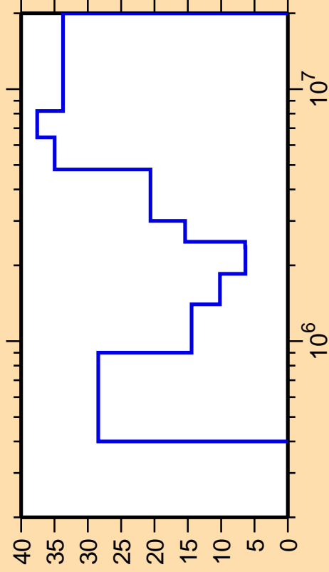
\Delta\sigma/\sigma vs. E for ^{87}\text{Br}(n,n_3)
