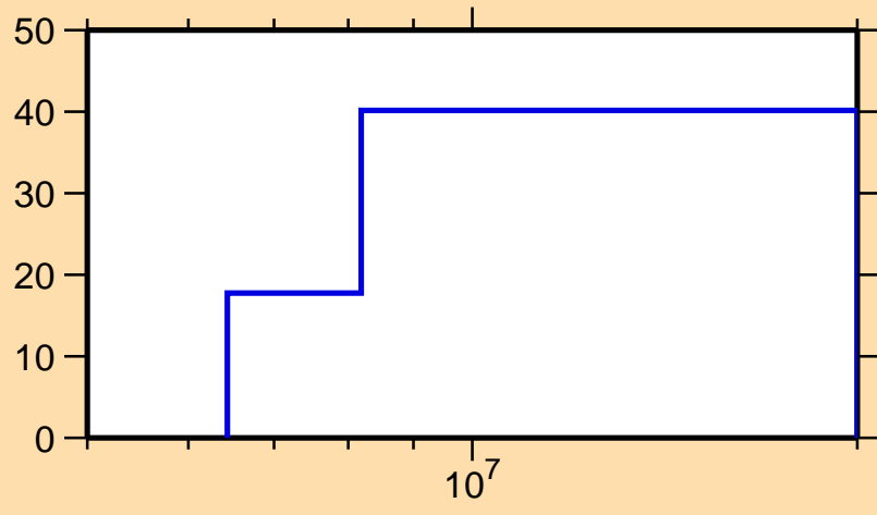
\Delta\sigma/\sigma vs. E for ^{87}\text{Br}(n,ncont.)
