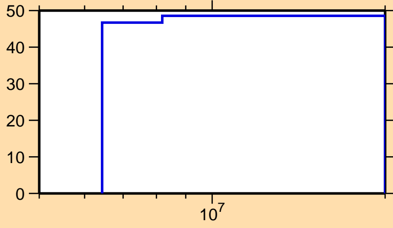
\Delta\sigma/\sigma vs. E for ^{87}\text{Br}(n,\gamma)
