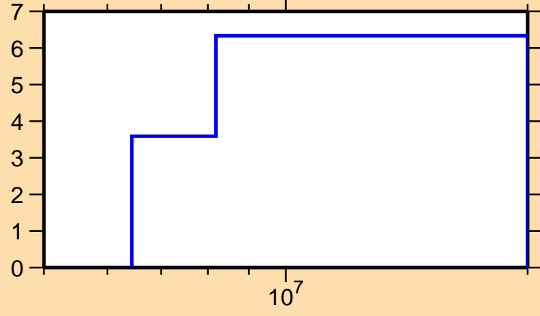
\Delta\sigma/\sigma vs. E for ^{87}\text{Br}(n,\text{tot.})
