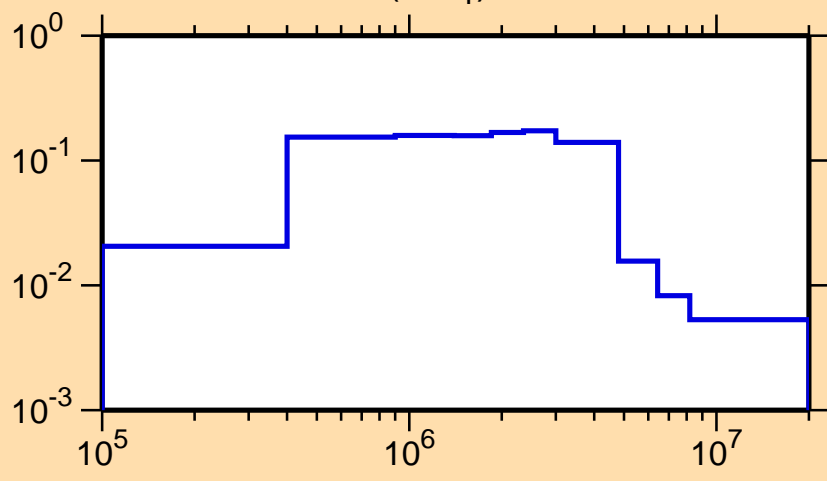
\sigma vs. E for ^{87}\text{Br}(n,n_1)
