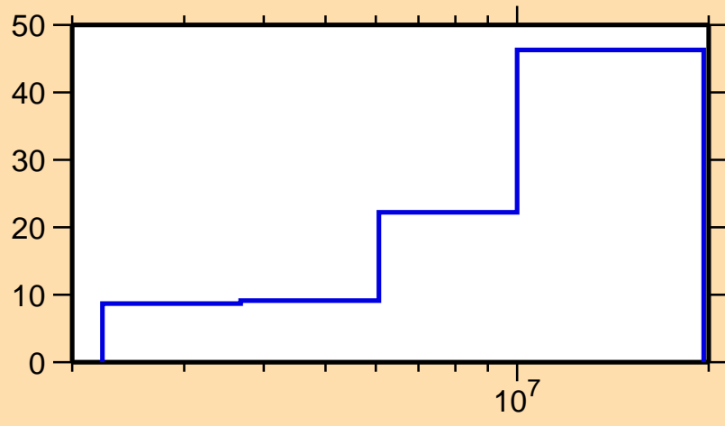
\Delta\sigma/\sigma vs. E for ^{88}\text{Br}(n,inel.)
