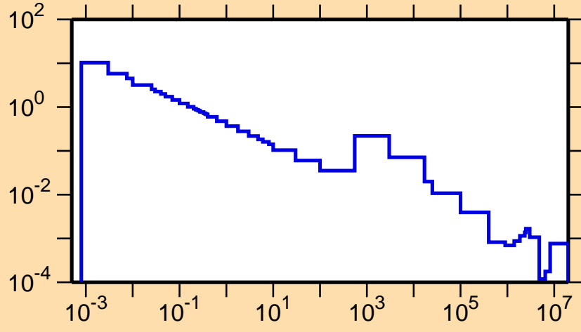
\sigma vs. E for ^{88}\text{Br}(n,\gamma)
