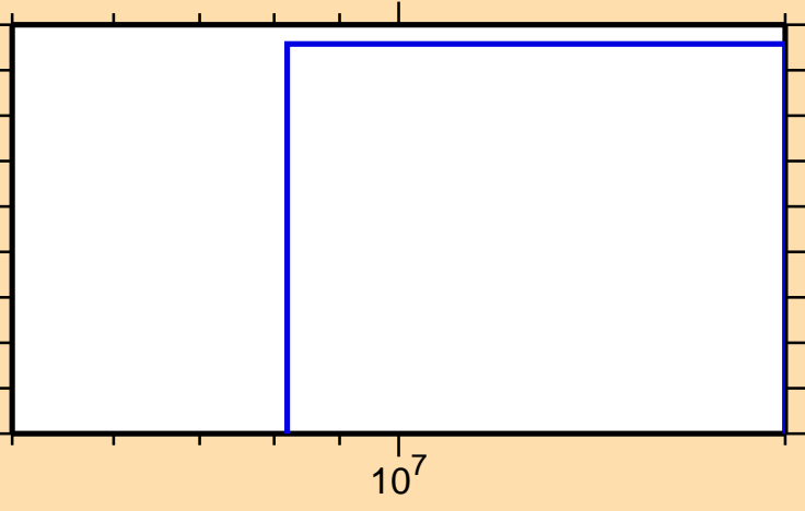
\sigma vs. E for ^{88}\text{Br}(n,\text{nd})
