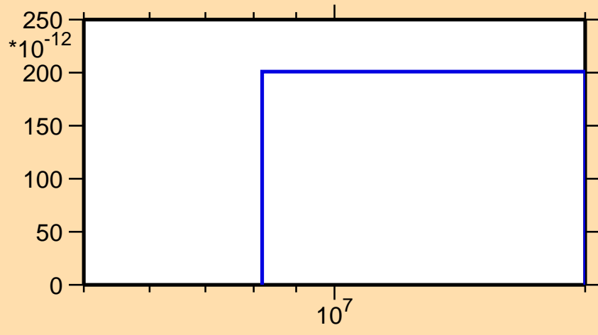
\sigma vs. E for ^{88}\text{Br}(n,2n\alpha)
