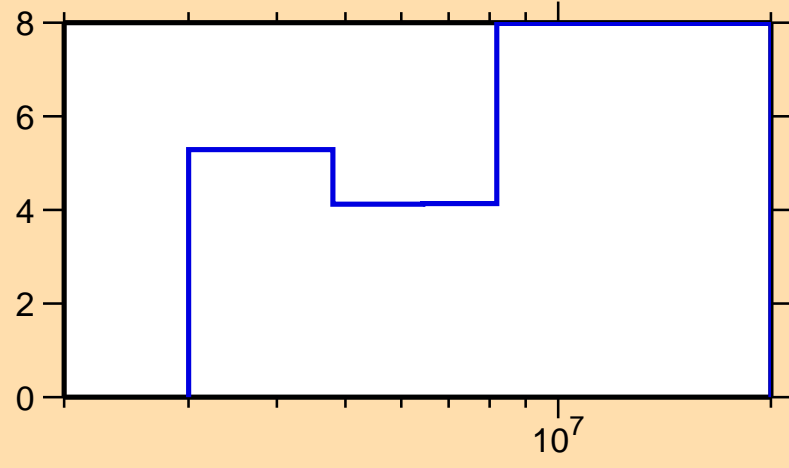
\Delta\sigma/\sigma vs. E for ^{88}\text{Br}(n,\text{tot.})
