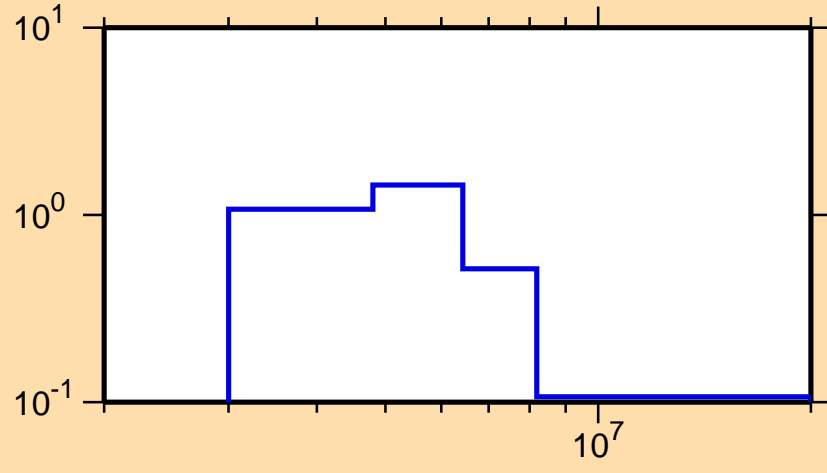
\sigma vs. E for ^{88}\text{Br}(n,n\text{cont.})
