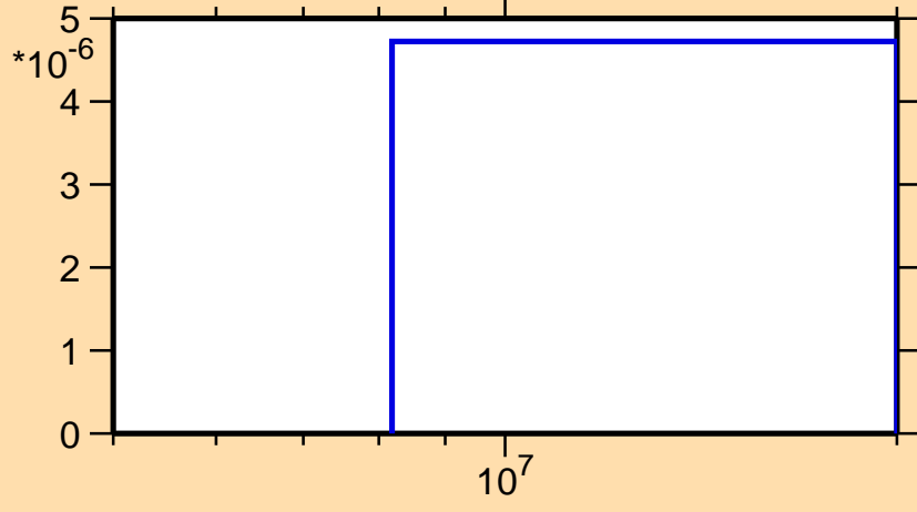
\sigma vs. E for ^{88}\text{Br}(n,\alpha)
