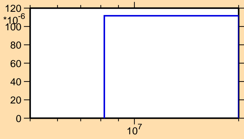
\sigma vs. E for ^{88}\text{Br}(n,d)
