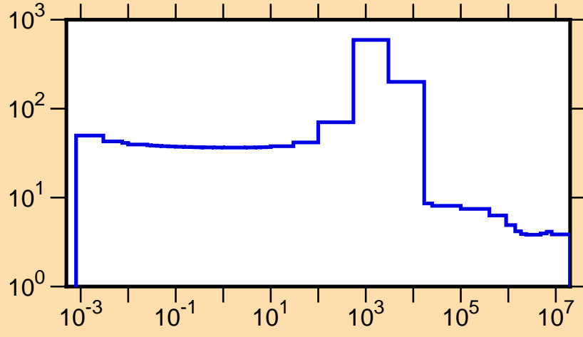
\sigma vs. E for ^{88}\text{Br}(n,\text{tot.})
