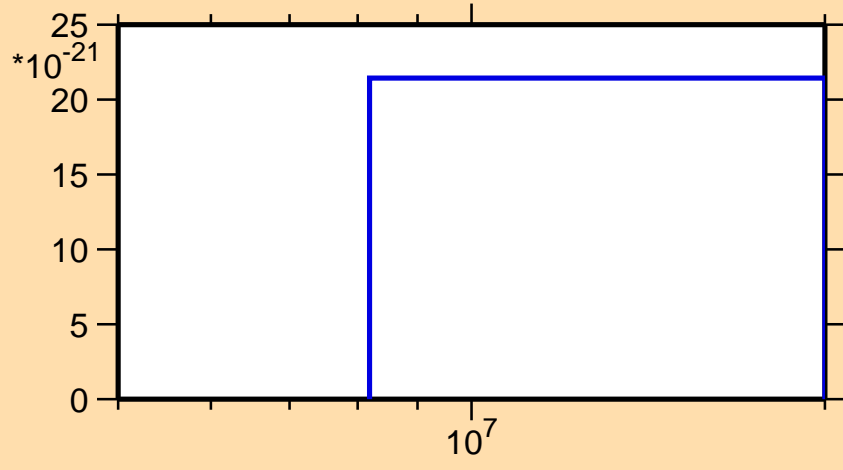
\sigma vs. E for ^{88}\text{Br} (mt 11)
