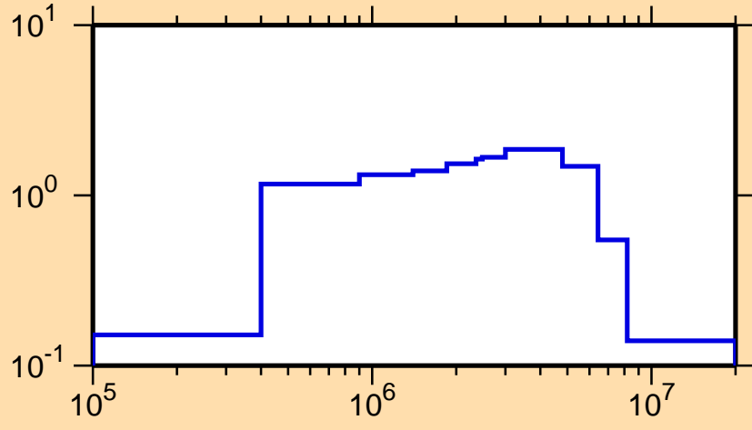
\sigma vs. E for ^{88}\text{Br}(n,\text{inel.})
