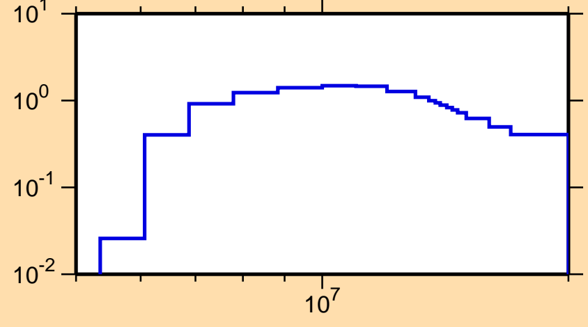
\sigma vs. E for ^{89}\text{Br}(n,2n)
