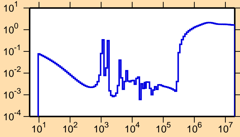
\sigma vs. E for ^{89}\text{Br}(n,\text{nonel.})
