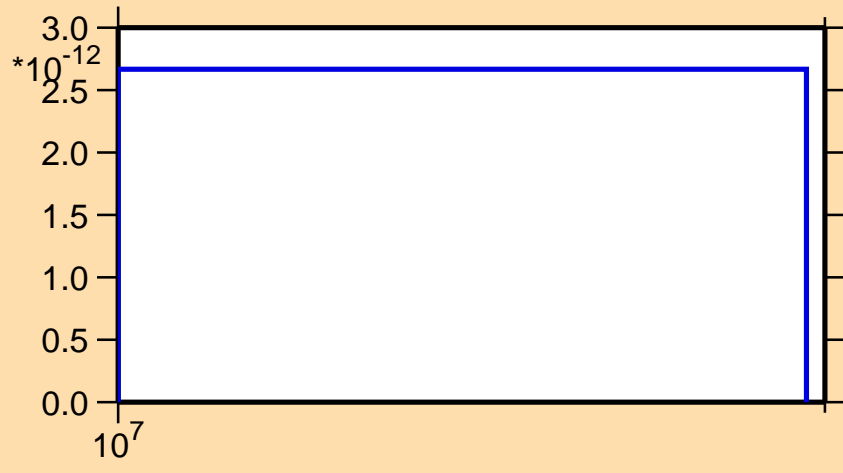
\sigma vs. E for ^{89}\text{Br}(n,2n\alpha)
