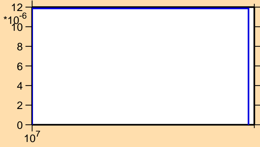
\sigma vs. E for ^{89}\text{Br}(n,np)
