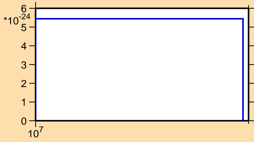
\sigma vs. E for ^{89}\text{Br} (mt 11)
