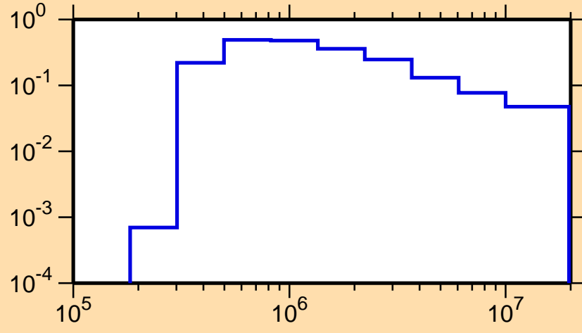
\sigma vs. E for ^{89}\text{Br}(n,n_1)
