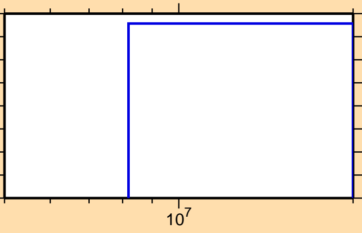
\sigma vs. E for ^{89}\text{Br}(n,\text{nd})
