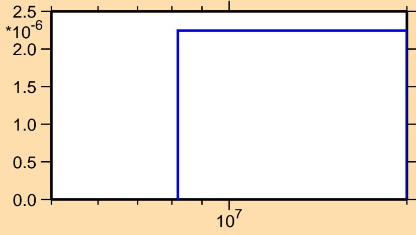
\sigma vs. E for ^{89}\text{Br}(n,\alpha)
