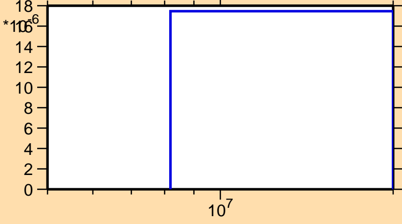
\sigma vs. E for ^{89}\text{Br}(n,t)
