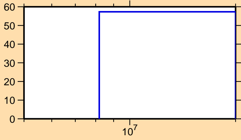
\Delta\sigma/\sigma vs. E for ^{89}\text{Br}(n,ncont.)
