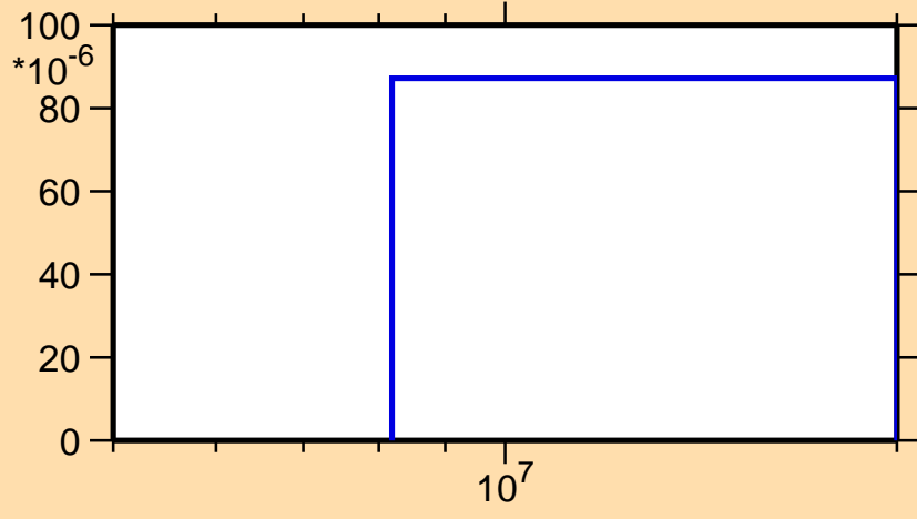
\sigma vs. E for ^{89}\text{Br}(n,d)
