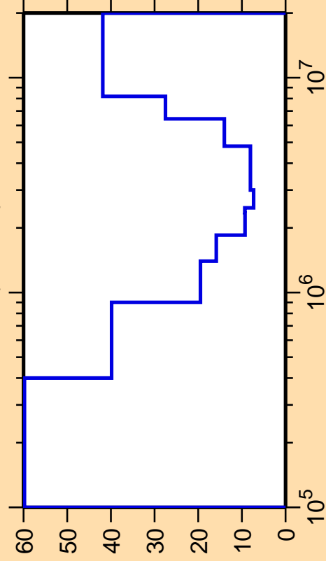
\Delta\sigma/\sigma vs. E for ^{89}\text{Br}(n,\text{inel.})
