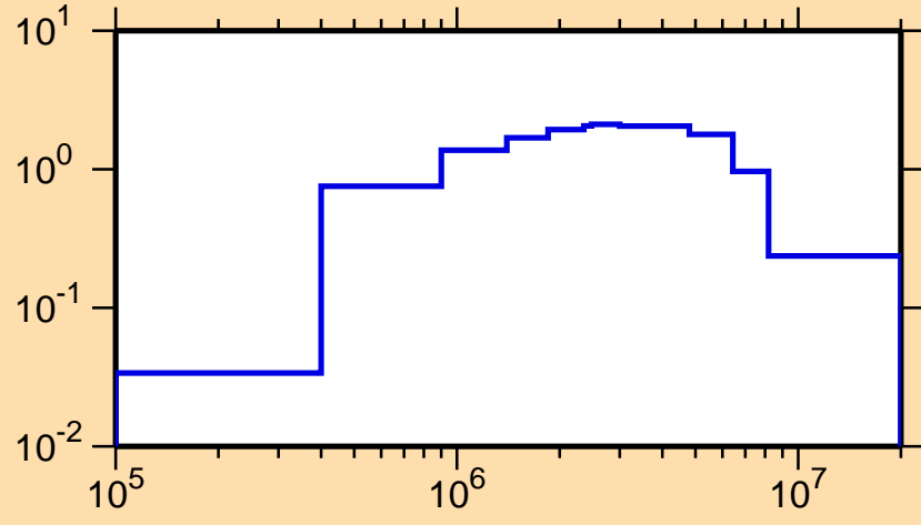
\sigma vs. E for ^{89}\text{Br}(n,\text{inel.})
