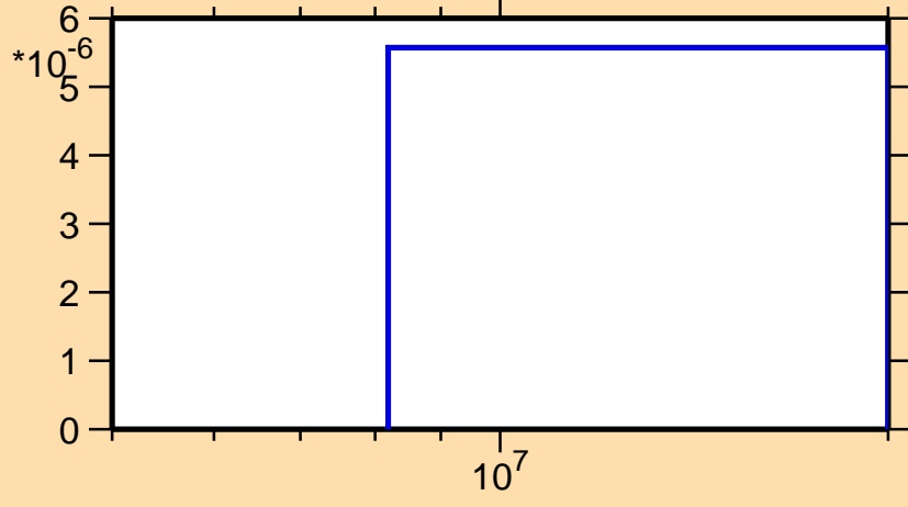
\sigma vs. E for ^{90}\text{Br}(n,np)
