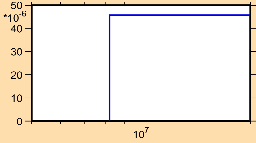
\sigma vs. E for ^{90}\text{Br}(n,d)
