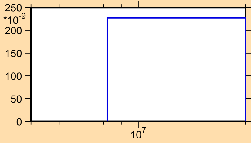
\sigma vs. E for ^{90}\text{Br}(n,\text{nd})
