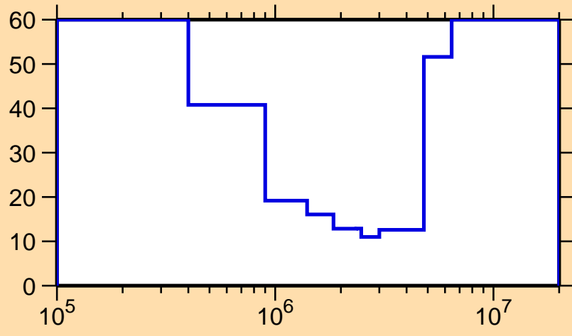
\Delta\sigma/\sigma vs. E for ^{90}\text{Br}(n,n\text{cont.})
