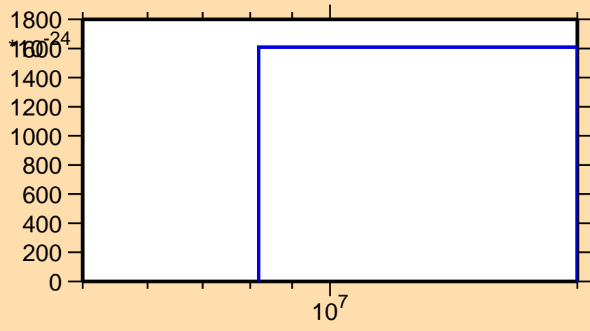
\sigma vs. E for ^{90}\text{Br} (mt 11)
