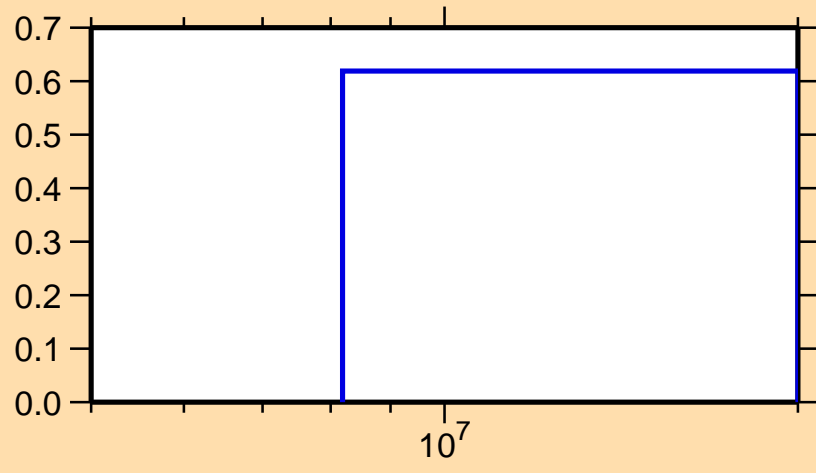
\sigma vs. E for ^{90}\text{Br}(n,3n)
