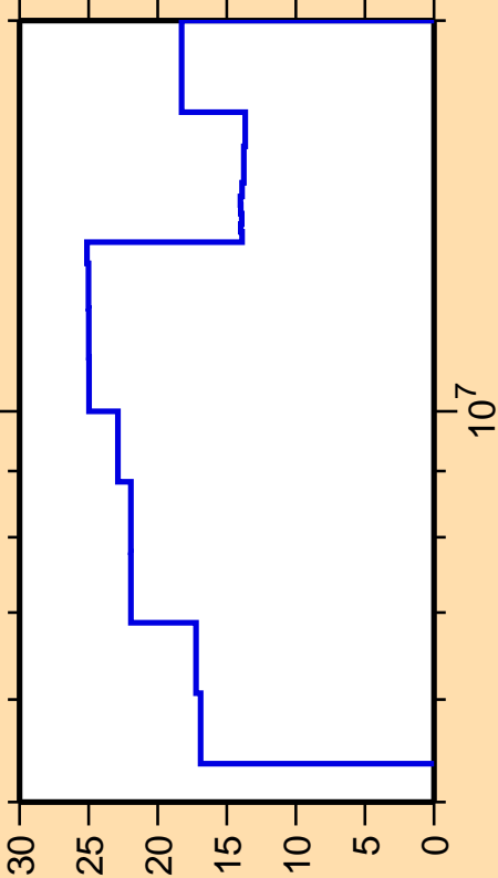
\Delta\sigma/\sigma vs. E for ^{10}\text{C}(n,\alpha)
