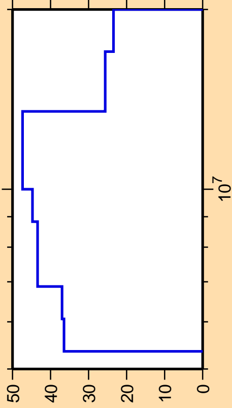
\Delta\sigma/\sigma vs. E for ^{10}\text{C}(n,\text{ncont.})
