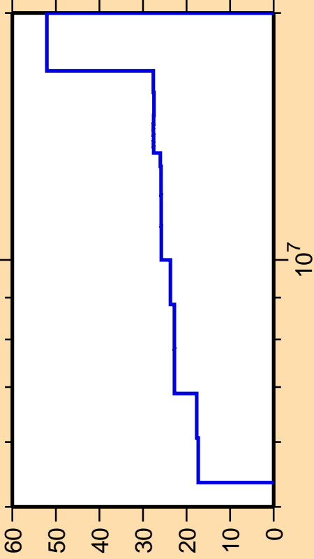
\Delta\sigma/\sigma vs. E for ^{10}\text{C}(n,p)
