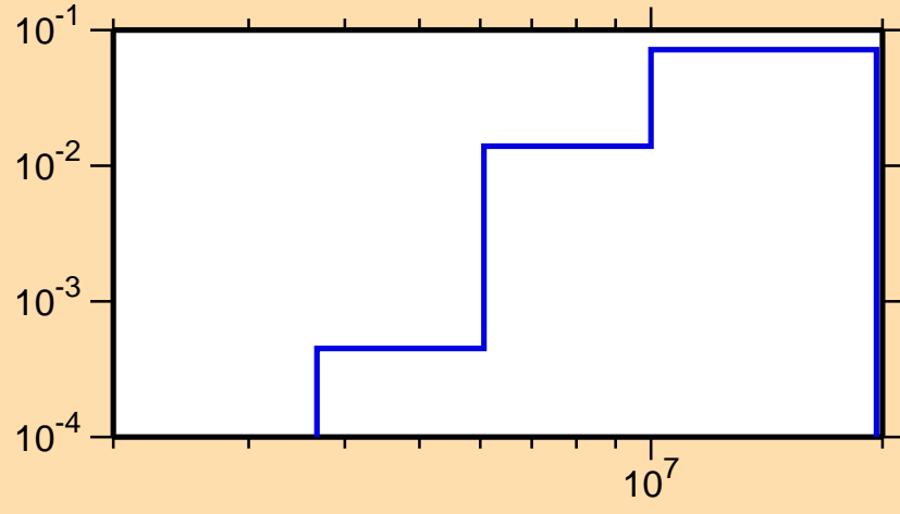
\sigma vs. E for ^{10}\text{C}(n,np)
