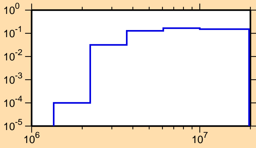
\sigma vs. E for ^{10}\text{C}(n,p\alpha)
