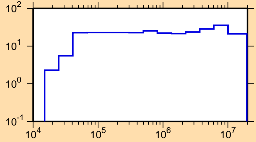
\Delta\sigma/\sigma vs. E for ^{10}\text{C}(n,\gamma)
