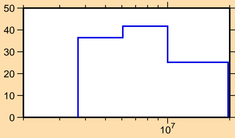
\Delta\sigma/\sigma vs. E for ^{10}\text{C}(n,ncont.)
