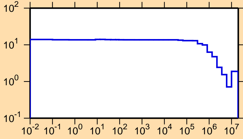
\Delta\sigma/\sigma vs. E for ^{10}\text{C}(n,el.)
