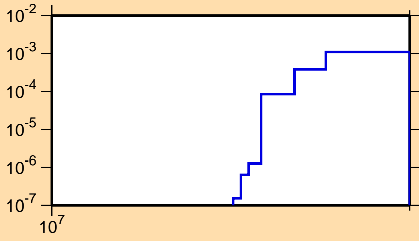
\sigma vs. E for ^{11}\text{C}(n,\text{pd})
