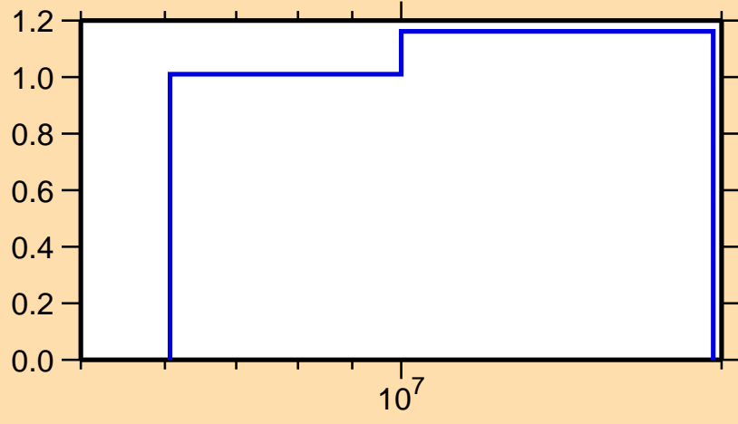
\Delta\sigma/\sigma vs. E for ^{11}\text{C}(n,tot.)
