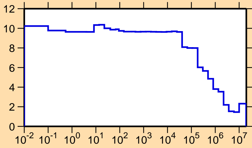
\Delta\sigma/\sigma vs. E for ^{11}\text{C}(n,el.)
