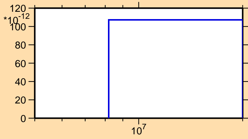
\sigma vs. E for ^{14}\text{C}(n,d)
