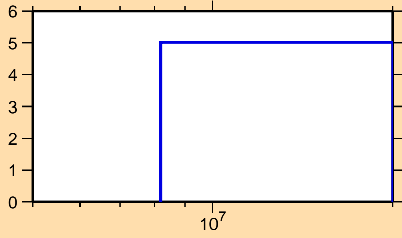
\Delta\sigma/\sigma vs. E for ^{15}\text{C}(n,n_1)
