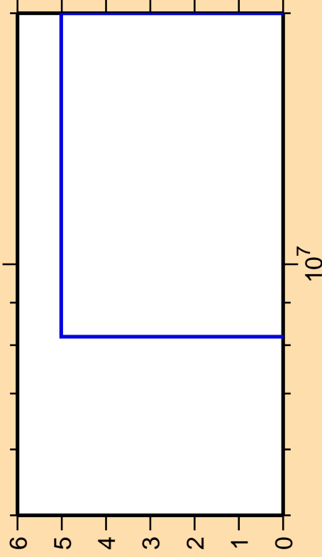
\Delta\sigma/\sigma vs. E for ^{15}\text{C}(n,n_1)
