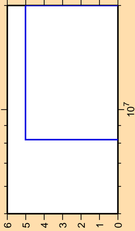
\Delta\sigma/\sigma vs. E for ^{15}\text{C}(n,n_1)
