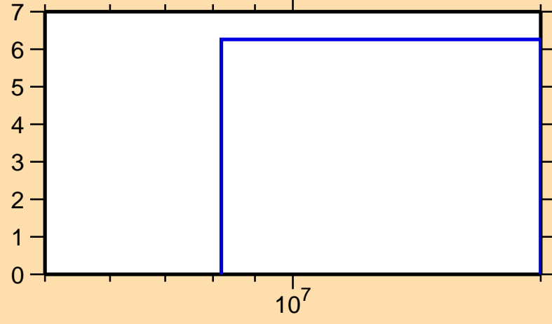
\Delta\sigma/\sigma vs. E for ^{15}\text{C}(n,2n)
