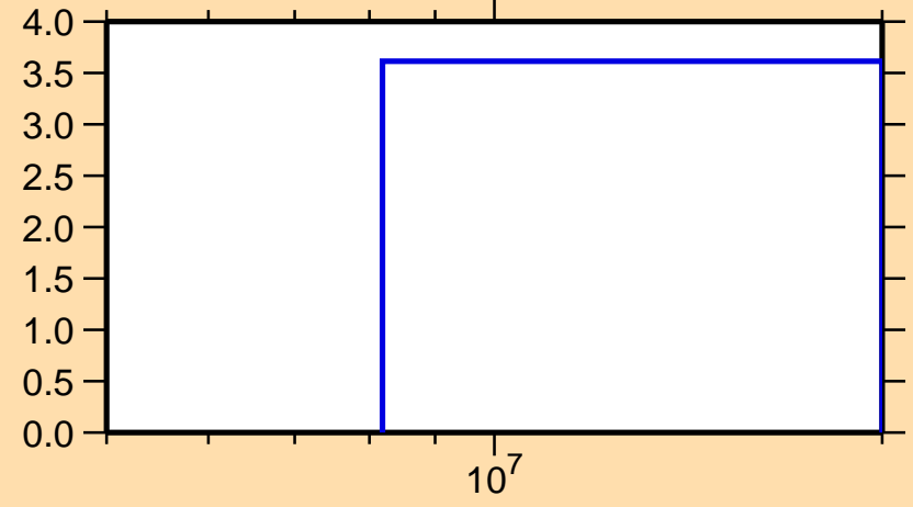
\Delta\sigma/\sigma vs. E for ^{15}\text{C}(n,\text{inel.})
