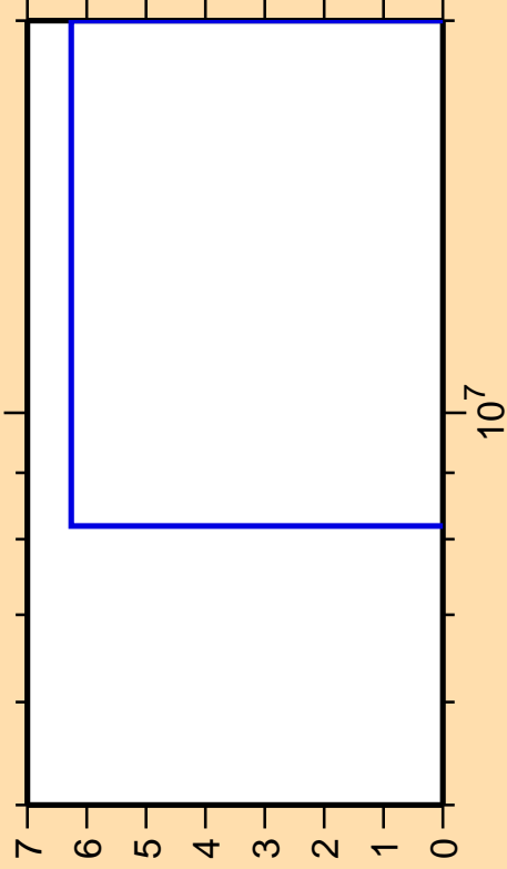
\Delta\sigma/\sigma vs. E for ^{15}\text{C}(n,2n)
