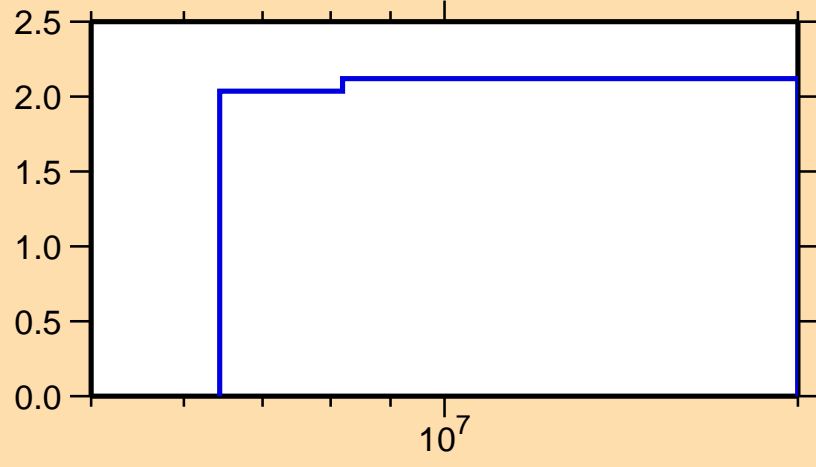
\Delta\sigma/\sigma vs. E for ^{40}\text{Ca}(n,n\text{nonel.})
