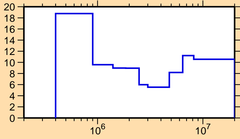
\Delta\sigma/\sigma vs. E for ^{40}\text{Ca}(n,p)
