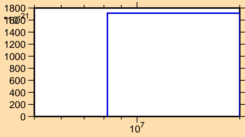
\sigma vs. E for ^{40}\text{Ca} (mt 34)
