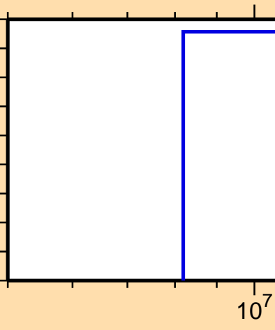
\sigma vs. E for ^{40}\text{Ca} (mt 34)
