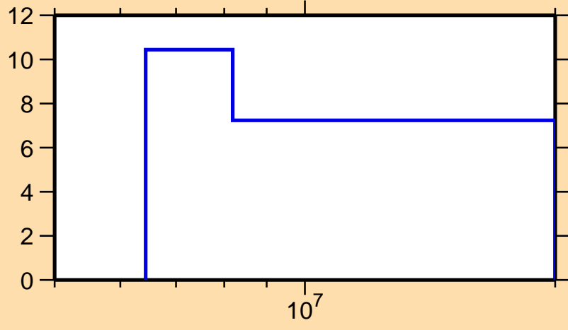
\Delta\sigma/\sigma vs. E for ^{40}\text{Ca}(n,ncont.)
