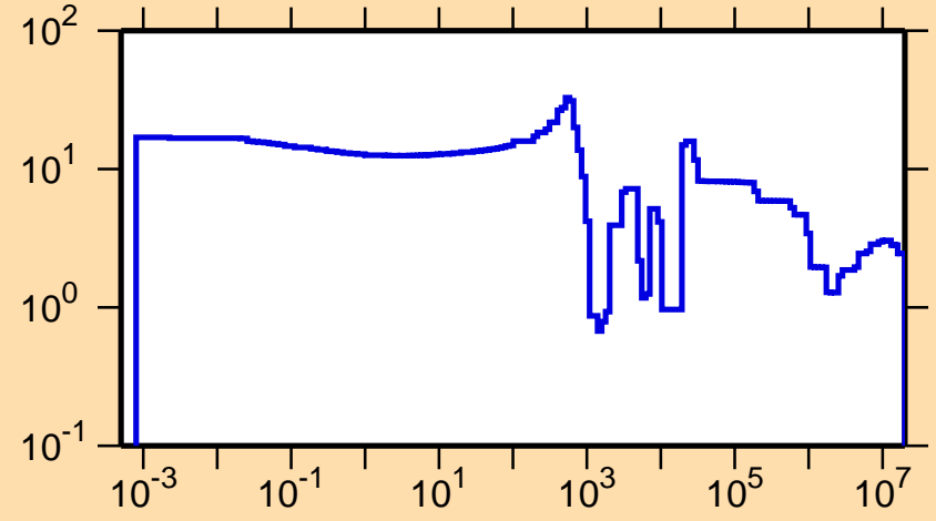
\Delta\sigma/\sigma vs. E for ^{41}\text{Ca}(n,\text{tot.})
