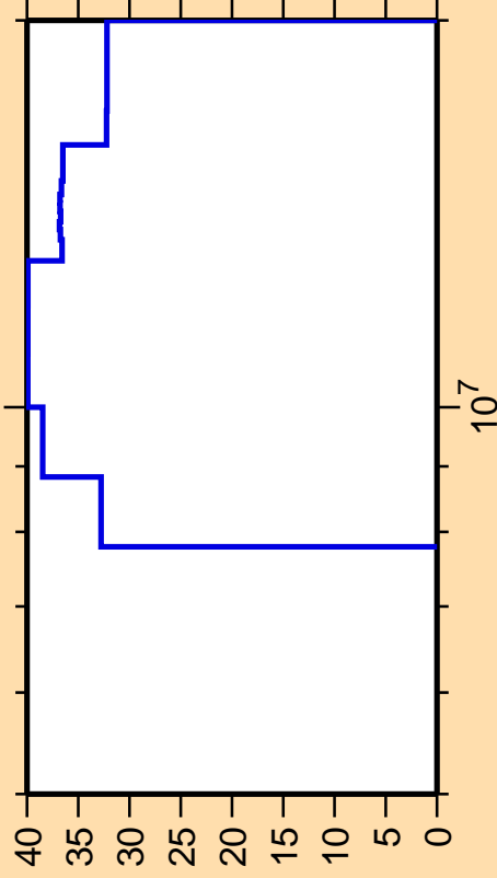
\Delta\sigma/\sigma vs. E for ^{41}\text{Ca}(n,\gamma)
