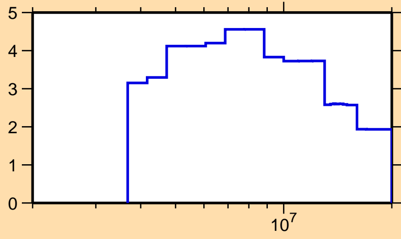
\Delta\sigma/\sigma vs. E for ^{41}\text{Ca}(n, el.)
