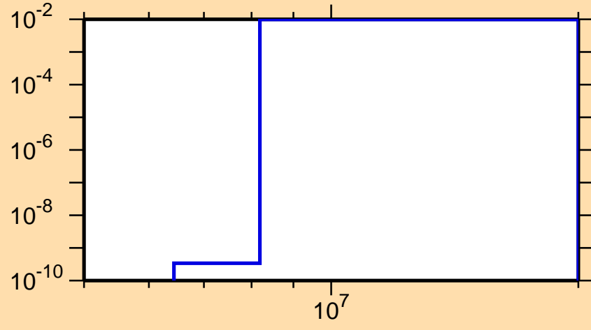
\sigma vs. E for ^{41}\text{Ca}(n,p\alpha)
