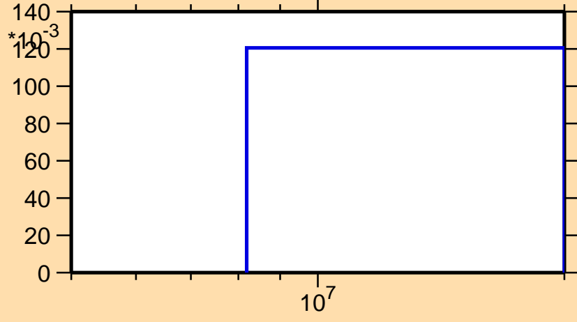
\sigma vs. E for ^{41}\text{Ca}(n,2n)
