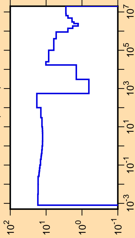
\Delta\sigma/\sigma vs. E for ^{41}\text{Ca}(n,\text{tot.})
