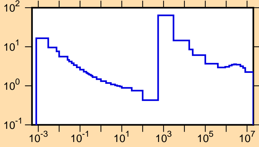
\sigma vs. E for ^{41}\text{Ca}(n,\text{tot.})
