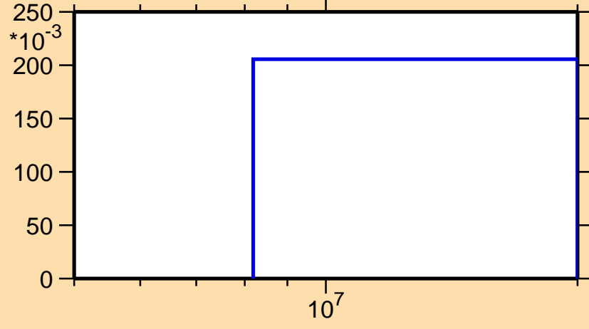
\sigma vs. E for ^{41}\text{Ca}(n,np)
