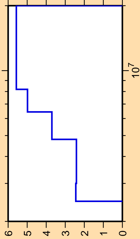
\Delta\sigma/\sigma vs. E for ^{42}\text{Ca}(n,n_3)
