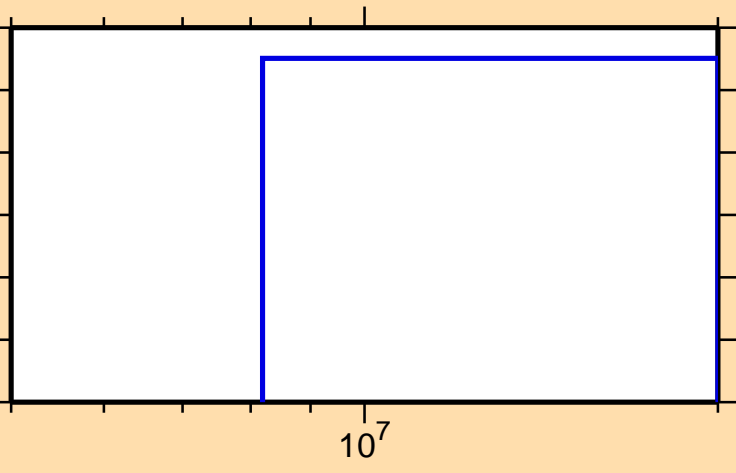
\sigma vs. E for ^{42}\text{Ca}(n,\text{pd})
