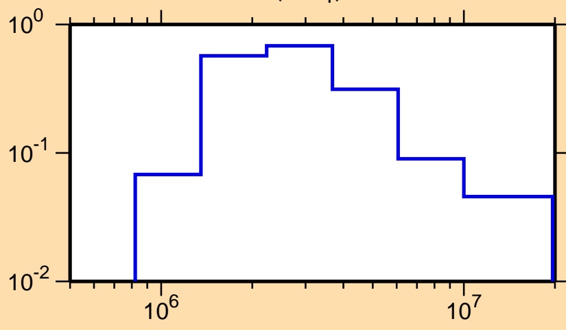
\sigma vs. E for ^{44}\text{Ca}(n,n_1)
