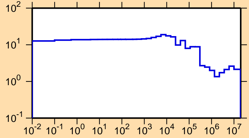
\Delta\sigma/\sigma vs. E for ^{44}\text{Ca}(n,\text{tot.})
