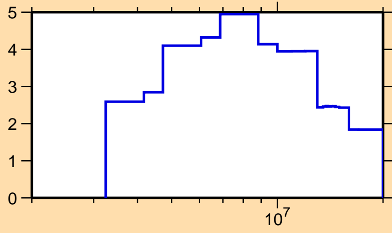
\Delta\sigma/\sigma vs. E for ^{45}\text{Ca}(n,el.)
