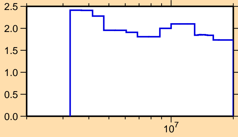
\Delta\sigma/\sigma vs. E for ^{45}\text{Ca}(n,n\text{onel.})
