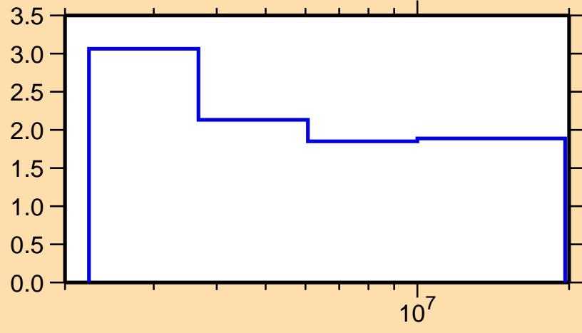
\Delta\sigma/\sigma vs. E for ^{45}\text{Ca}(n,n\text{nonel.})
