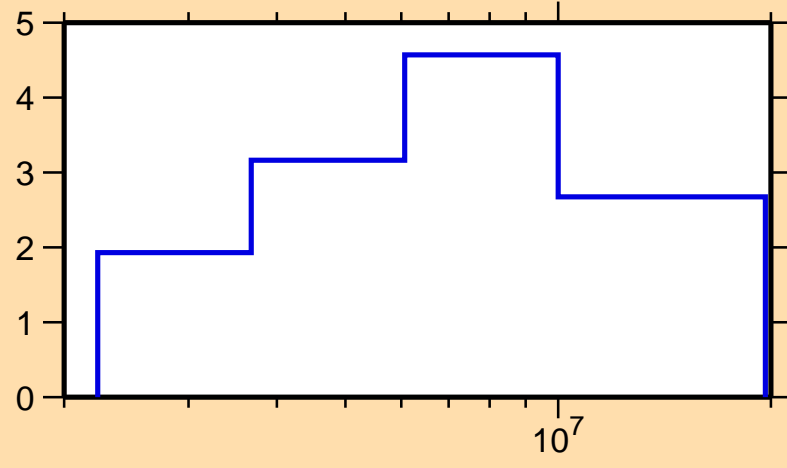
\Delta\sigma/\sigma vs. E for ^{45}\text{Ca}(n,\text{el.})
