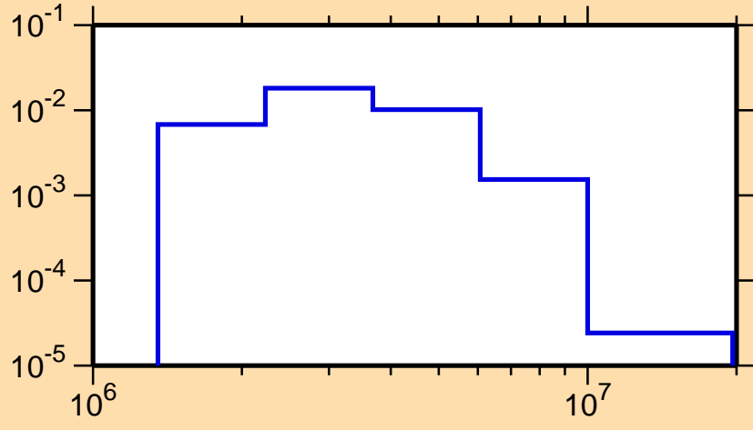
\sigma vs. E for ^{45}\text{Ca}(n,n_4)
