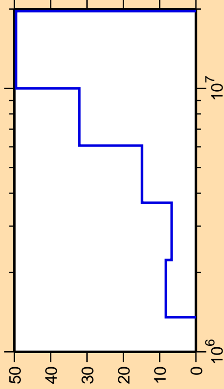
\Delta\sigma/\sigma vs. E for ^{45}\text{Ca}(n,n_4)
