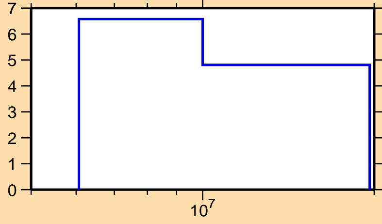
\Delta\sigma/\sigma vs. E for ^{45}\text{Ca}(n,2n)
