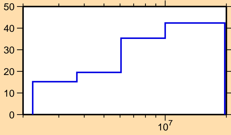
\Delta\sigma/\sigma vs. E for ^{45}\text{Ca}(n,\gamma)
