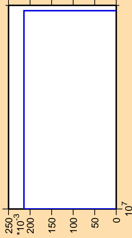
\Delta\sigma/\sigma vs. E for ^{45}\text{Ca}(n,\text{He}3)
