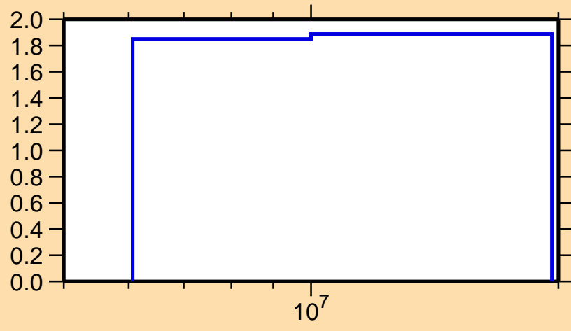
\Delta\sigma/\sigma vs. E for ^{45}\text{Ca}(n,\text{nonel.})
