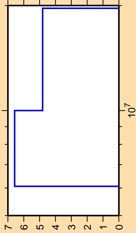
\Delta\sigma/\sigma vs. E for ^{45}\text{Ca}(n,2n)
