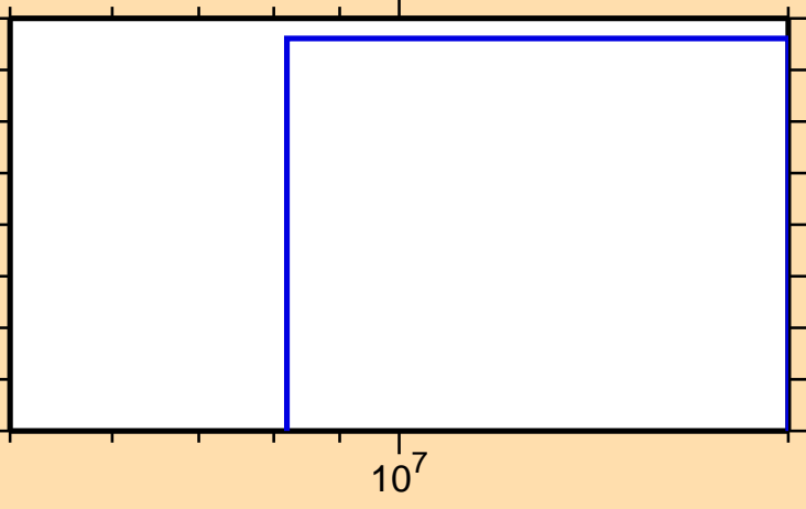
\sigma vs. E for ^{45}\text{Ca}(n,n\alpha)
