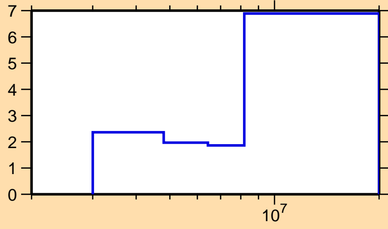
\Delta\sigma/\sigma vs. E for ^{45}\text{Ca}(n,\text{inel.})
