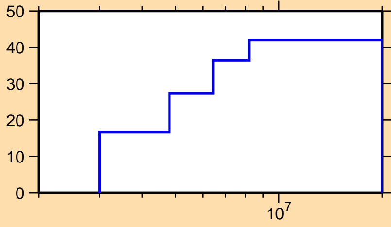
\Delta\sigma/\sigma vs. E for ^{45}\text{Ca}(n,\gamma)
