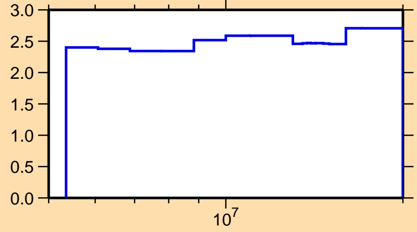
\Delta\sigma/\sigma vs. E for ^{46}\text{Ca}(n,n\text{onel.})
