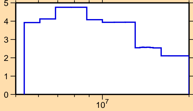
\Delta\sigma/\sigma vs. E for ^{46}\text{Ca}(n,\text{el.})
