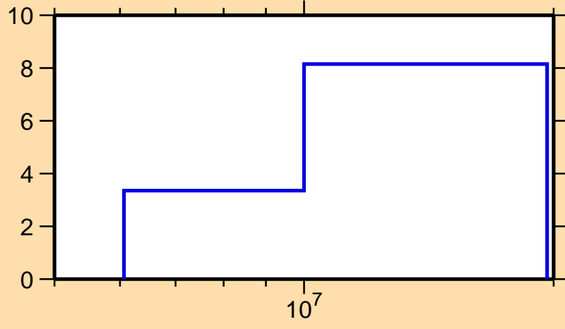
\Delta\sigma/\sigma vs. E for ^{46}\text{Ca}(n,ncont.)
