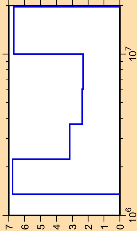
\Delta\sigma/\sigma vs. E for ^{46}\text{Ca}(n,\text{inel.})
