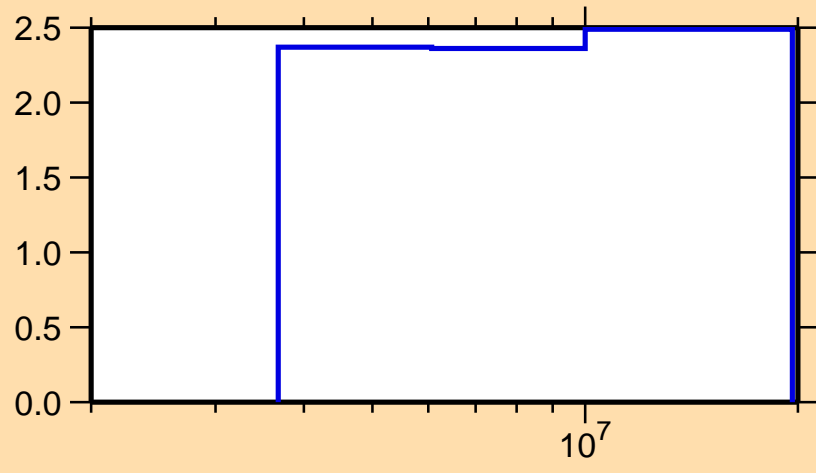
\Delta\sigma/\sigma vs. E for ^{46}\text{Ca}(n,n\text{nonel.})
