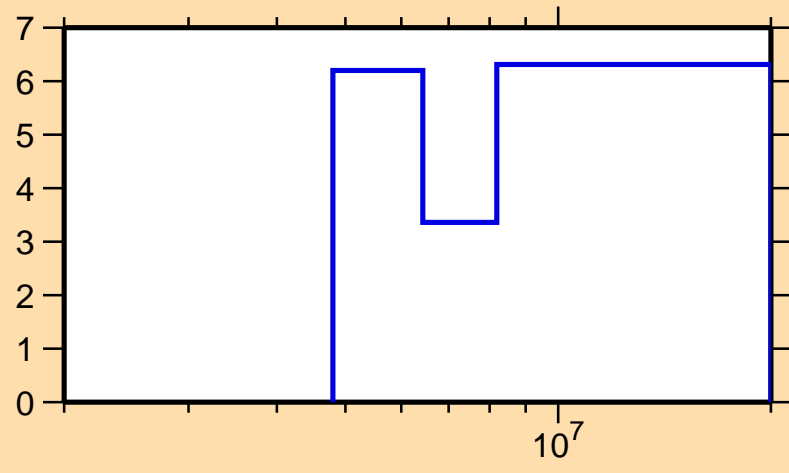
\Delta\sigma/\sigma vs. E for ^{46}\text{Ca}(n,n\text{cont.})
