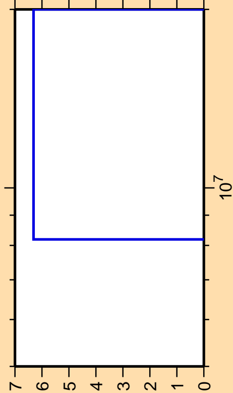
\Delta\sigma/\sigma vs. E for ^{46}\text{Ca}(n,n\text{cont.})
