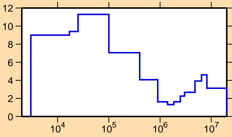
\Delta\sigma/\sigma vs. E for ^{46}\text{Ca}(n,\text{el.})
