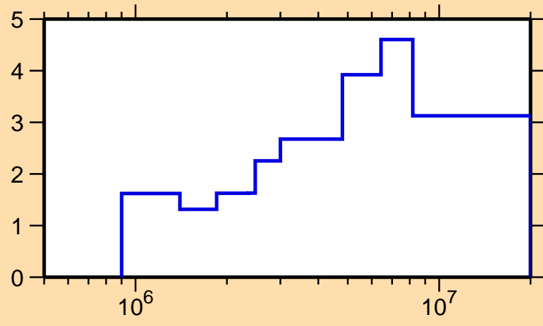
\Delta\sigma/\sigma vs. E for ^{46}\text{Ca}(n,\text{el.})
