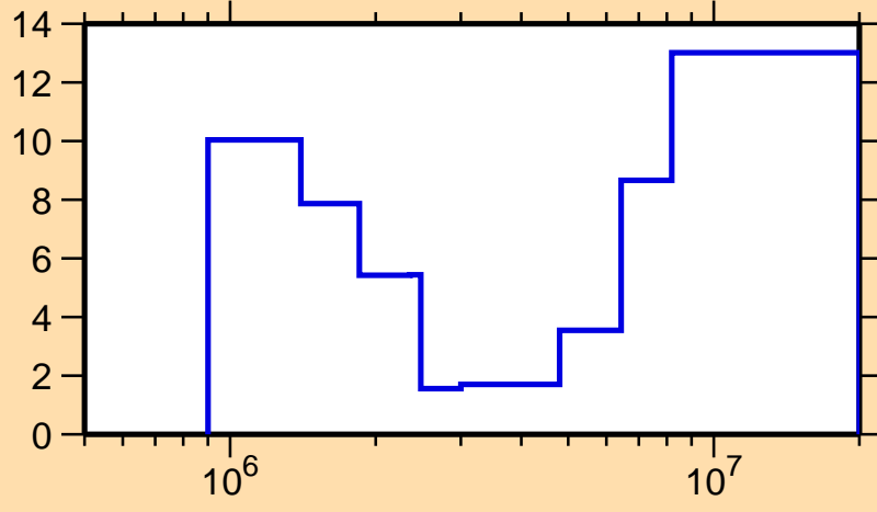
\Delta\sigma/\sigma vs. E for ^{46}\text{Ca}(n,n_1)
