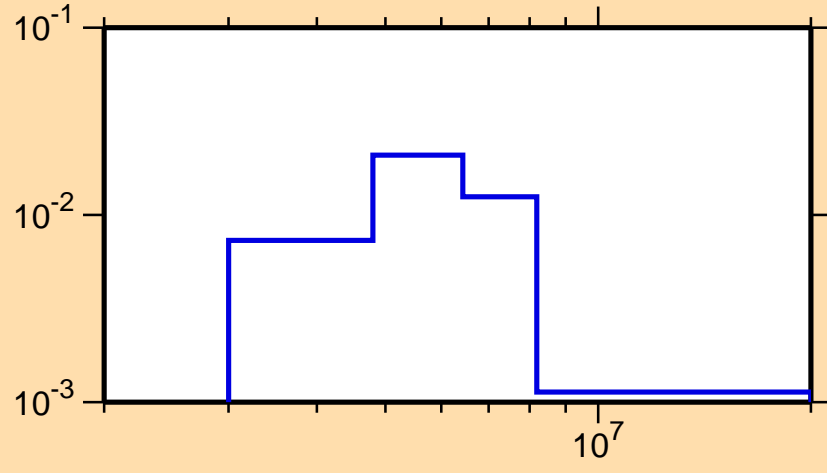
\sigma vs. E for ^{46}\text{Ca}(n,n_4)
