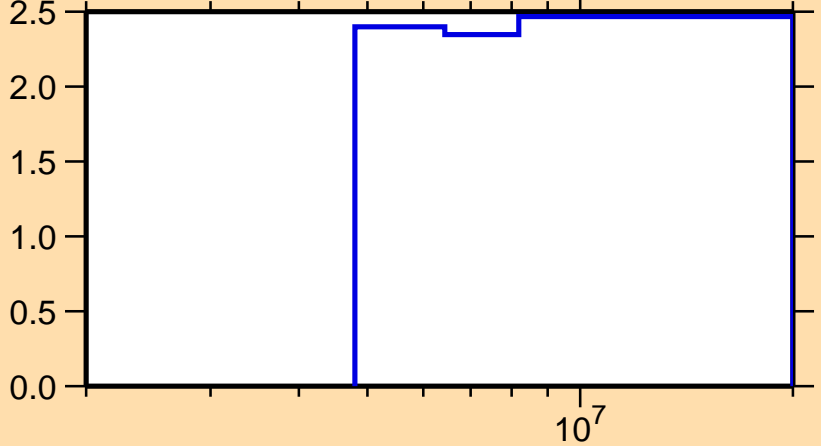
\Delta\sigma/\sigma vs. E for ^{46}\text{Ca}(n,n\text{nonel.})
