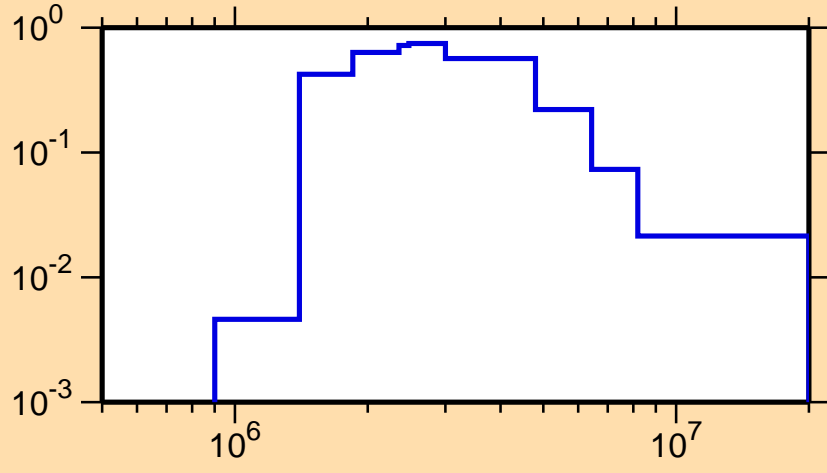
\sigma vs. E for ^{46}\text{Ca}(n,n_1)
