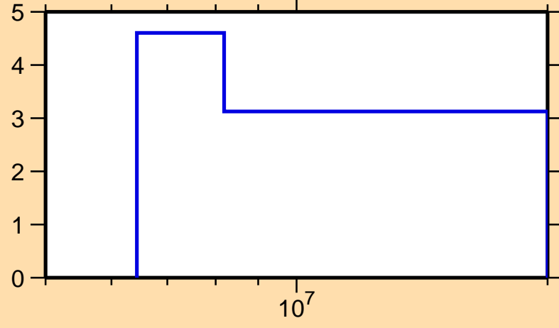
\Delta\sigma/\sigma vs. E for ^{46}\text{Ca}(n,el.)
