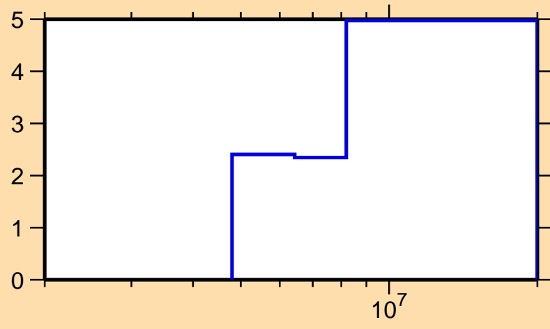
\Delta\sigma/\sigma vs. E for ^{46}\text{Ca}(n,\text{inel.})
