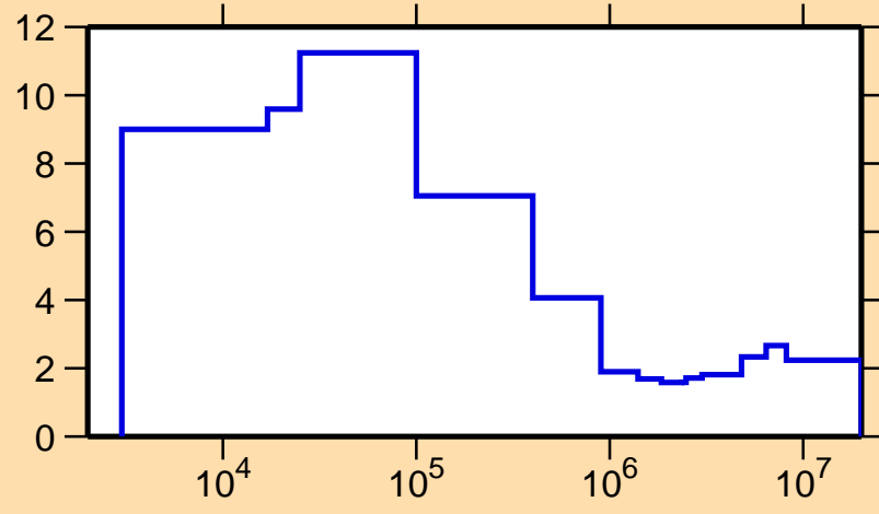
\Delta\sigma/\sigma vs. E for ^{46}\text{Ca}(n,\text{tot.})
