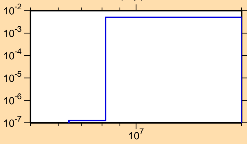
\sigma vs. E for ^{46}\text{Ca}(n,p)
