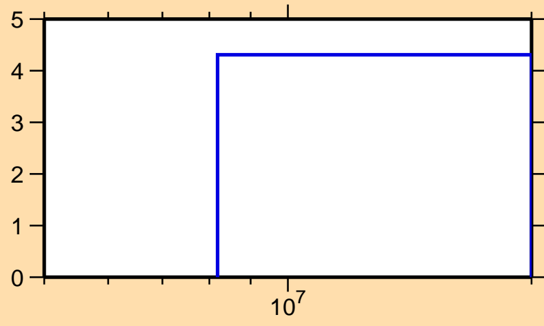
\Delta\sigma/\sigma vs. E for ^{46}\text{Ca}(n,2n)
