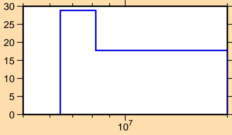
\Delta\sigma/\sigma vs. E for ^{46}\text{Ca}(n,p)
