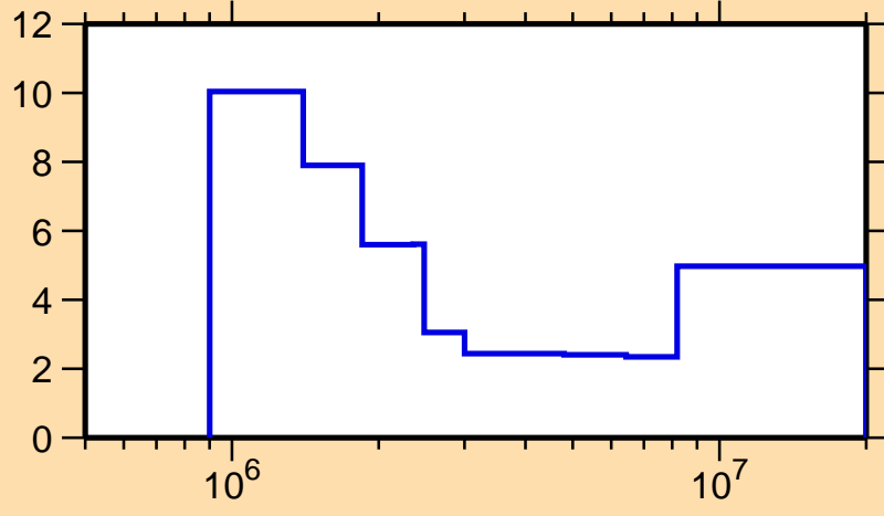
\Delta\sigma/\sigma vs. E for ^{46}\text{Ca}(n,\text{inel.})
