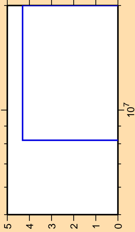
\Delta\sigma/\sigma vs. E for ^{46}\text{Ca}(n,2n)
