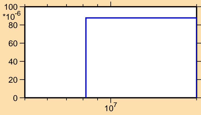
\sigma vs. E for ^{46}\text{Ca}(n,d)
