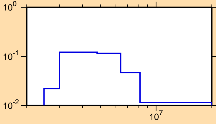
\sigma vs. E for ^{46}\text{Ca}(n,n_3)
