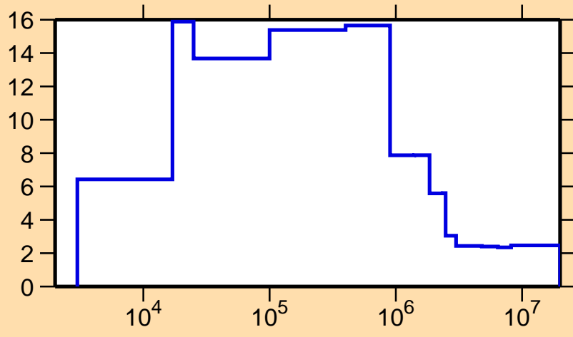
\Delta\sigma/\sigma vs. E for ^{46}\text{Ca}(n,\text{nonel.})
