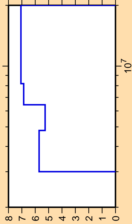
\Delta\sigma/\sigma vs. E for ^{46}\text{Ca}(n,n_4)
