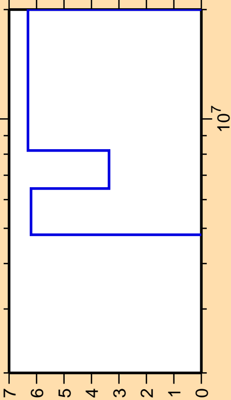
\Delta\sigma/\sigma vs. E for ^{46}\text{Ca}(n,n\text{cont.})
