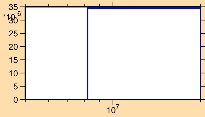
\sigma vs. E for ^{46}\text{Ca}(n,np)
